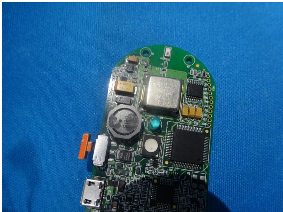
EUT RF Module with shield
