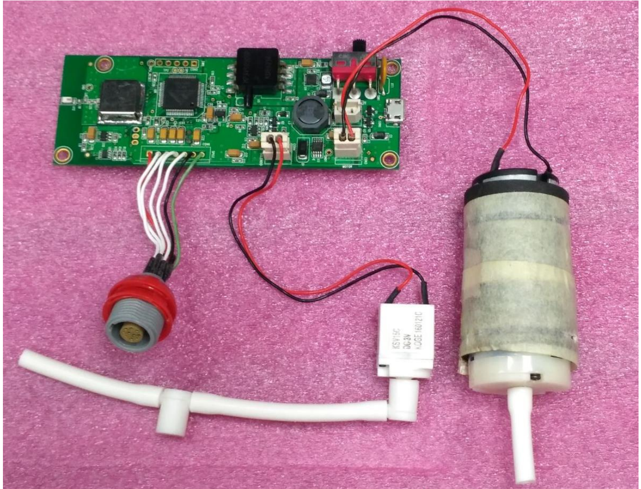
PCB With Connected Air Pump and Solenoid
