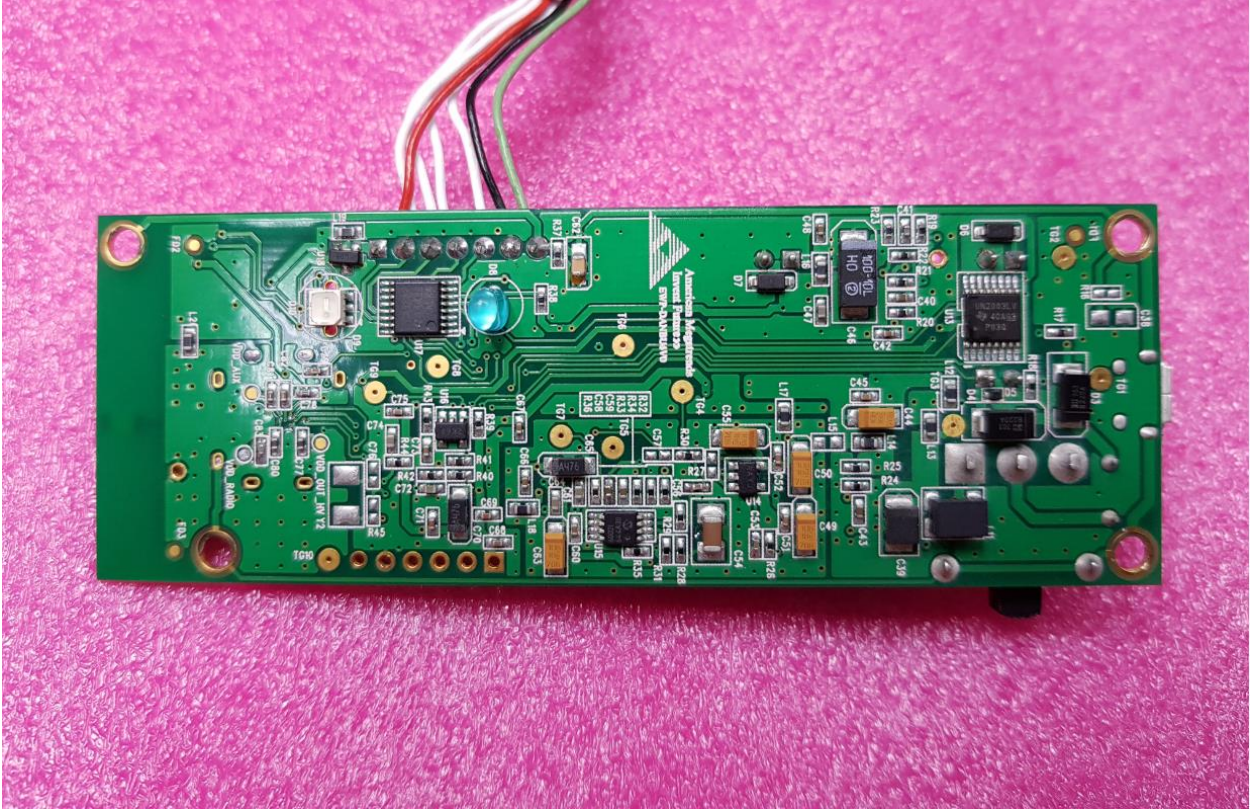
EUT PCB Top View
