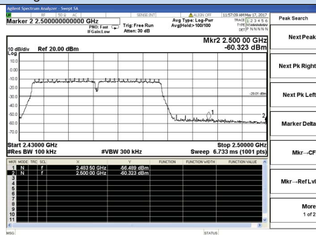
802.11n(HT40)-High channel
