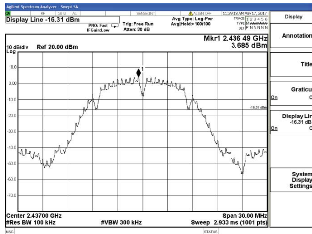
802.11b_Middle Channel
