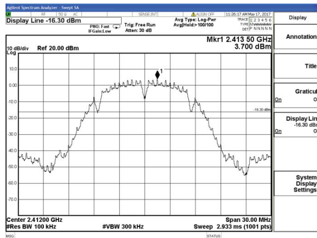
802.11b_Low Channel
