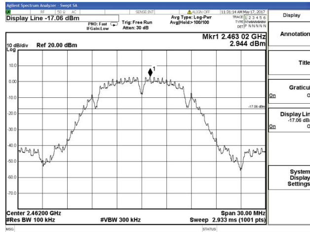
802.11b_High Channel
