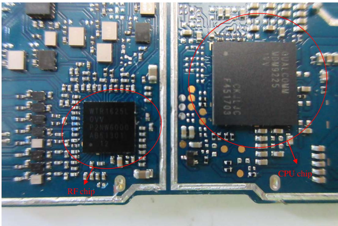
4. CPU/RF chip view
