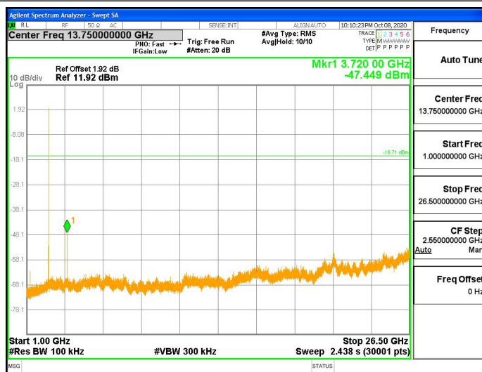
BLE_BT4.0_Ant1_2480_1000~26500
