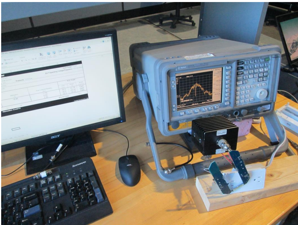
Conducted EMI at the Antenna Port – (2.4GHz radio)
