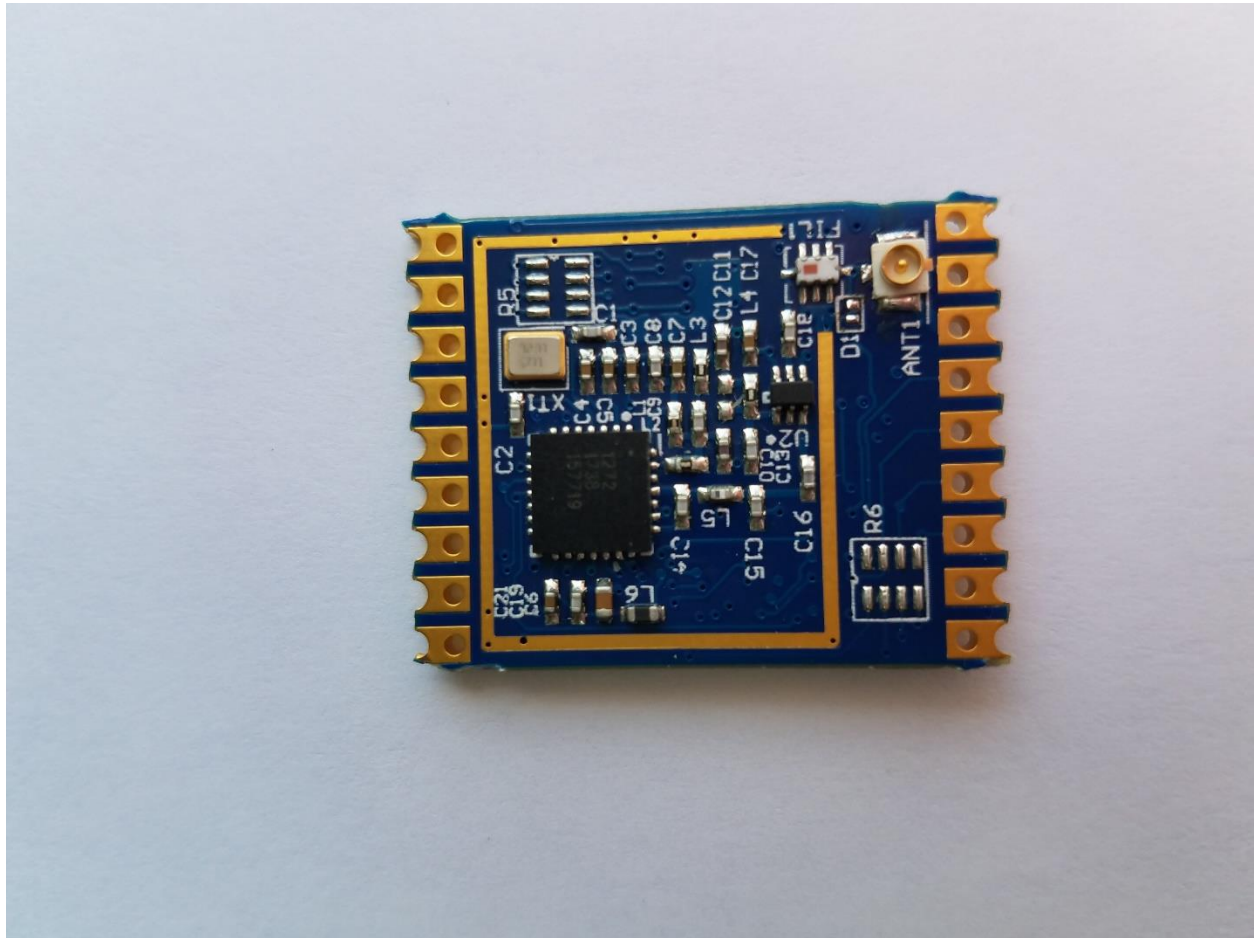
Figure 2 - EUT Top, Shield removed
