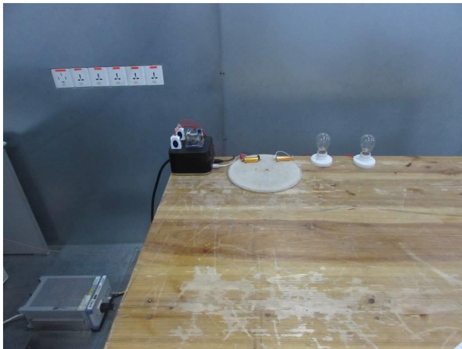
Conducted Emissions at Mains Terminals
