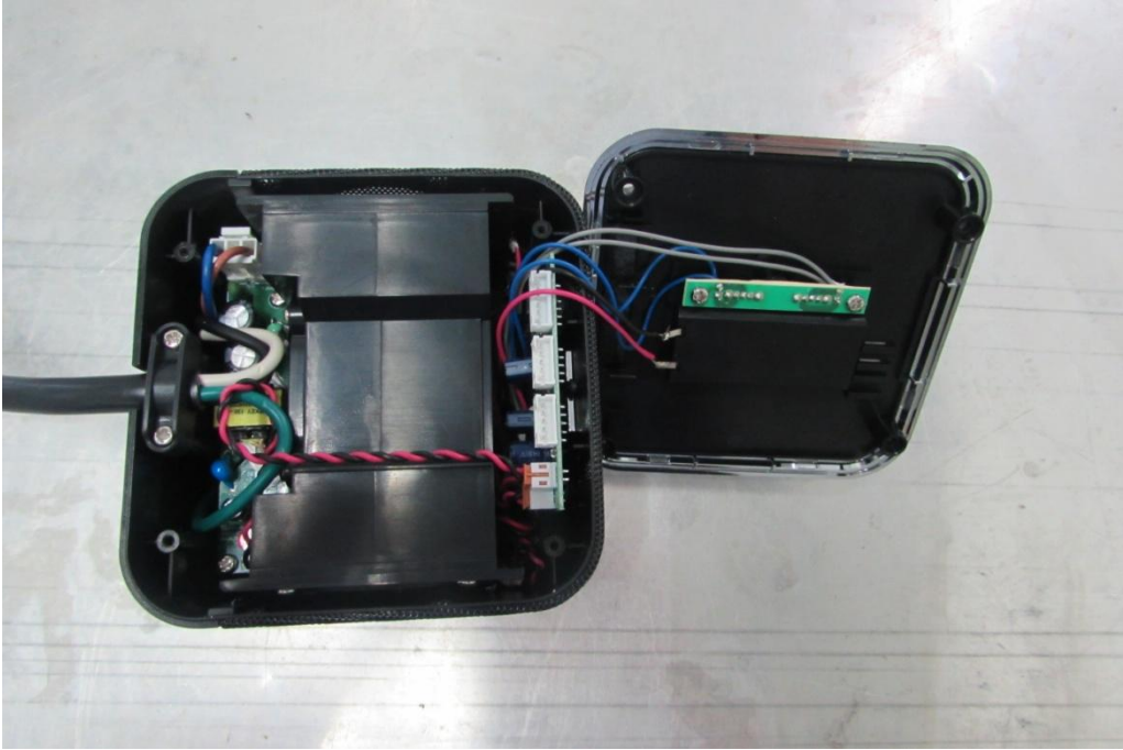
Internal view of model BPEBL
