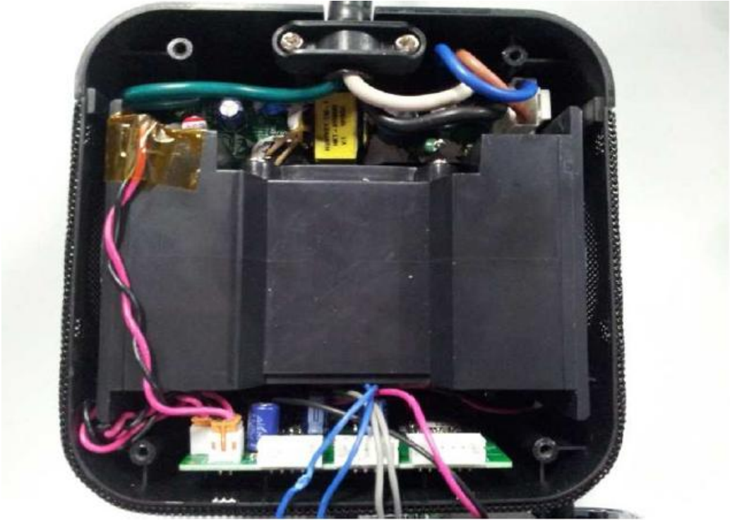
Internal view of model BPEBL
