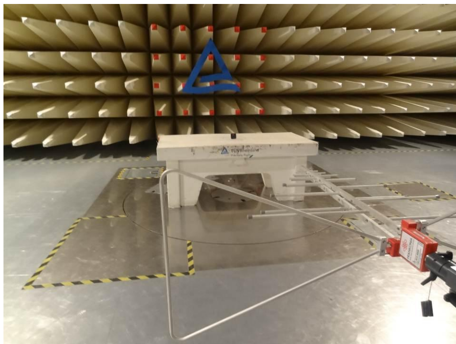
Test setup
