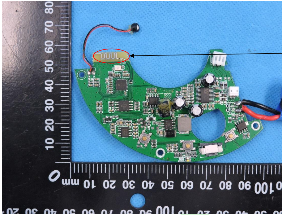
BT Antenna
