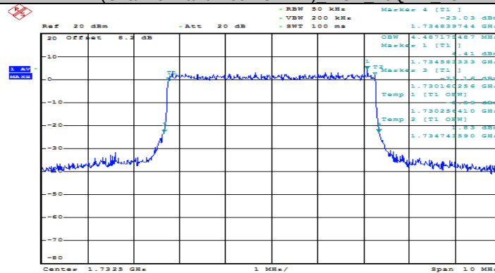
(Channel Bandwidth: 5 MHz) MCH 16QAM 25RB#0
