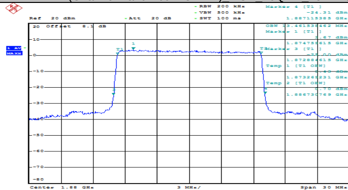
(Channel Bandwidth:15 MHz) MCH 16QAM 75RB#0
