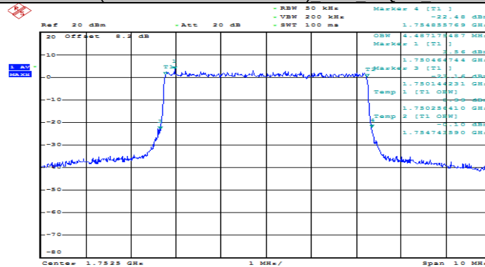
(Channel Bandwidth: 5 MHz) HCH 16QAM 25RB#0
