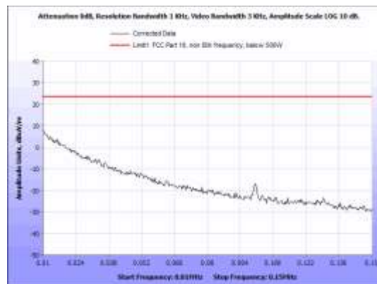
Figure 11: Field Strength Limits, V Unit, 0.01 - 0.15 MHz, Parallel
