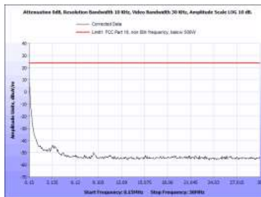
Figure 12: Field Strength Limits, V Unit, 0.15 - 30 MHz, Perpendicular
