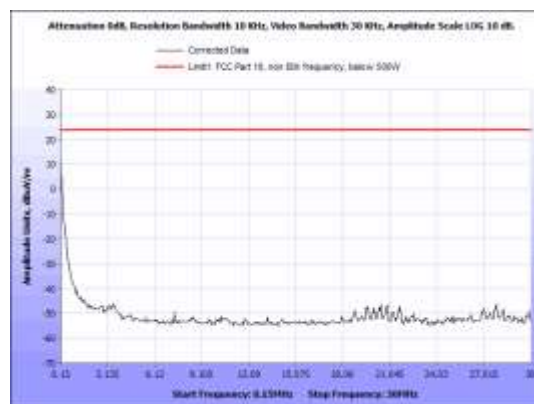
Figure 13: Field Strength Limits, V Unit, 0.15 - 30 MHz, Parallel
