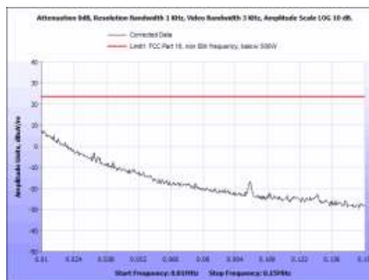
Figure 10: Field Strength Limits, V Unit, 0.01 - 0.15 MHz, Perpendicular
