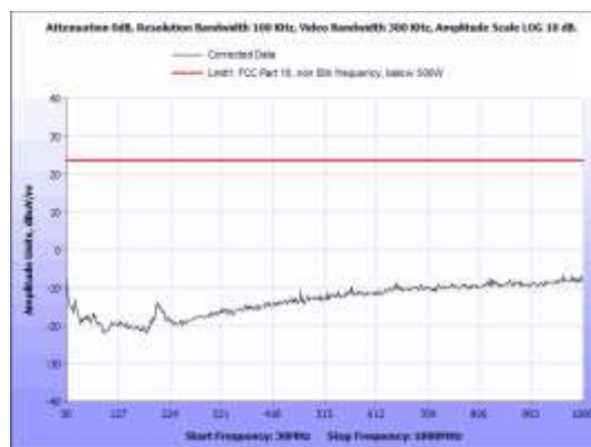
Figure 14: Field Strength Limits, V Unit, 30 - 1000 MHz
