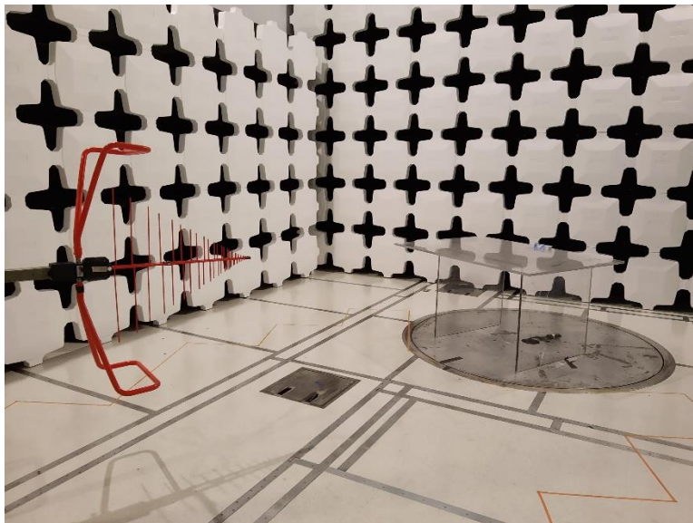
Figure 4: Radiated Emission: Limits of Electromagnetic Radiation Disturbance, setup above 30 MHz
