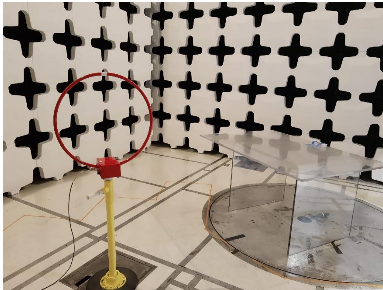
Figure 3: Radiated Emission: Limits of Electromagnetic Radiation Disturbance, setup below 30MHz - Perpendicular
