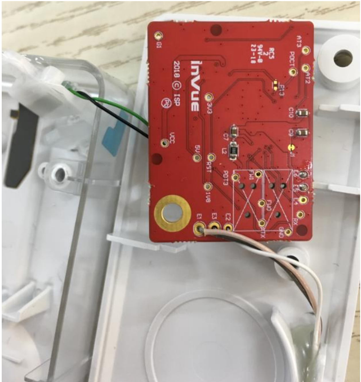
PCBA Bottom View Taken out from Plastic
