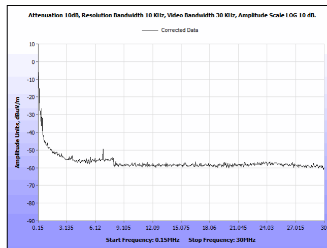
Plot 7. Radiated Emission – (150 kHz – 30 MHz), Vertical Unit, Pen Charging Plot
