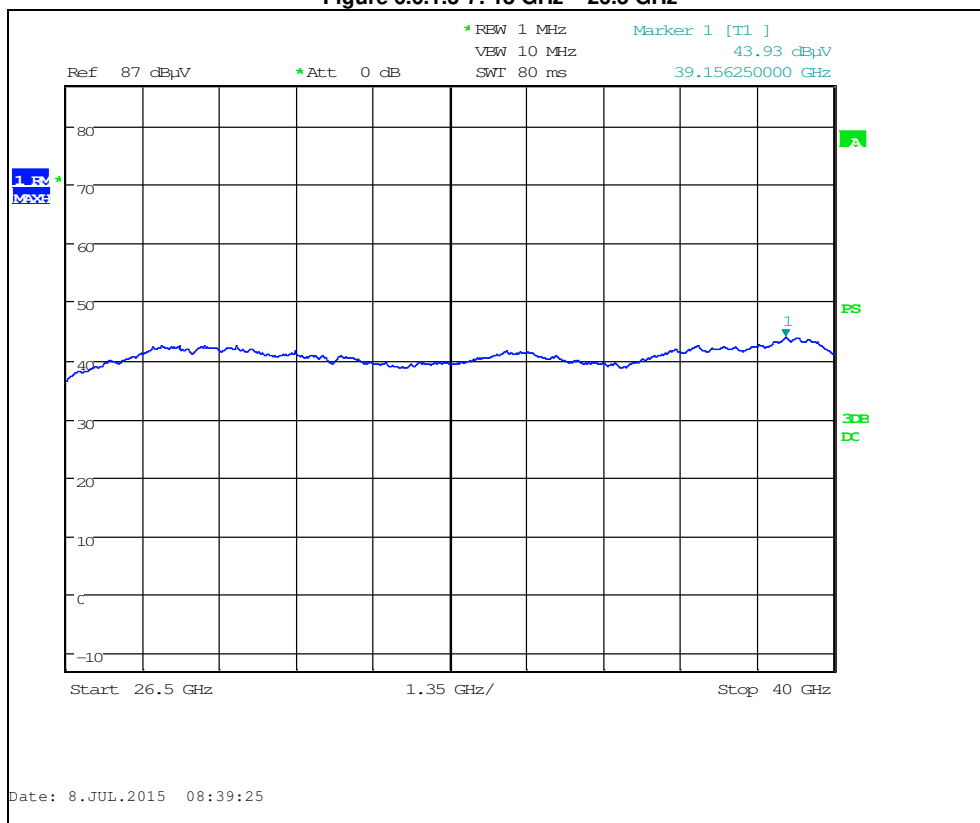
Figure 6.6.1.3-8: 26.5 GHz – 40 GHz
