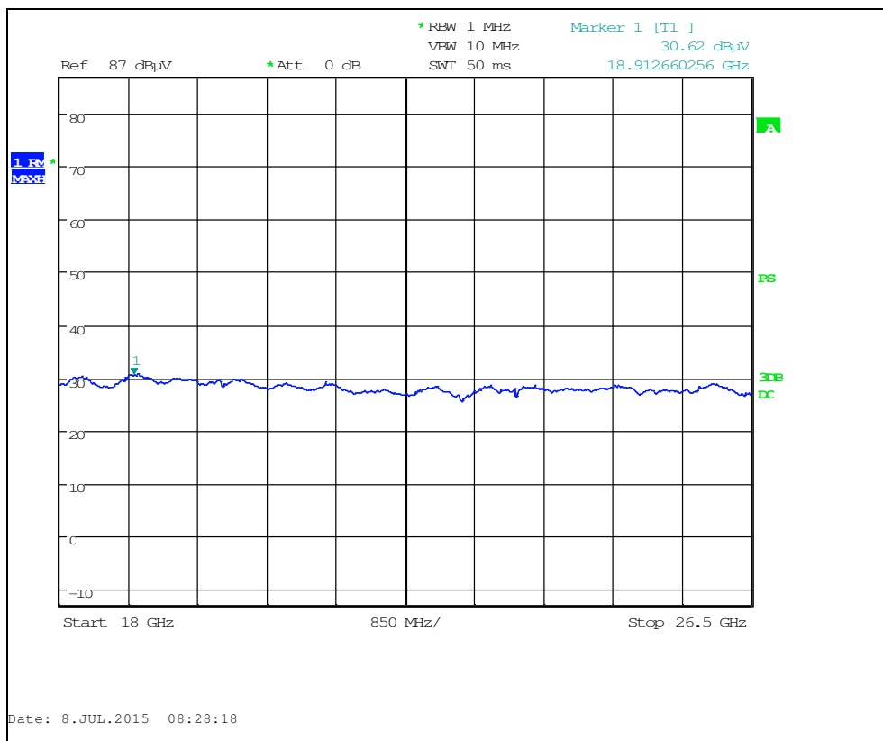
Figure 6.6.1.3-7: 18 GHz – 26.5 GHz
