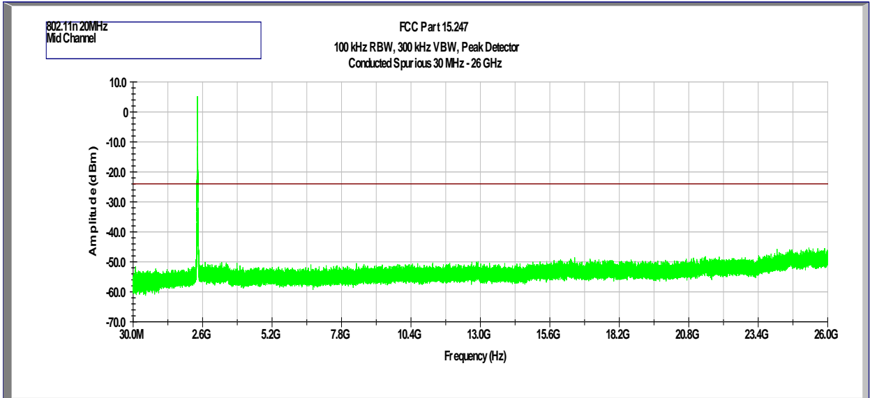
Plot 4.8 Tx @ 2437MHz 802.11n, 20MHz
