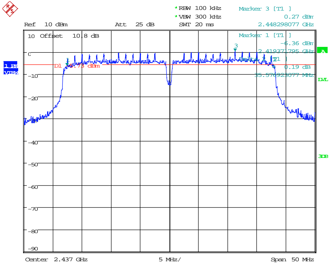
Plot 1.11 – 6dB Bandwidth (FCC)
