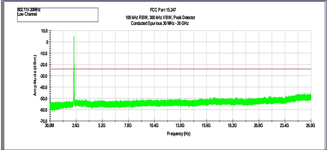
Plot 4.7 Tx @ 2412MHz 802.11n, 20MHz
