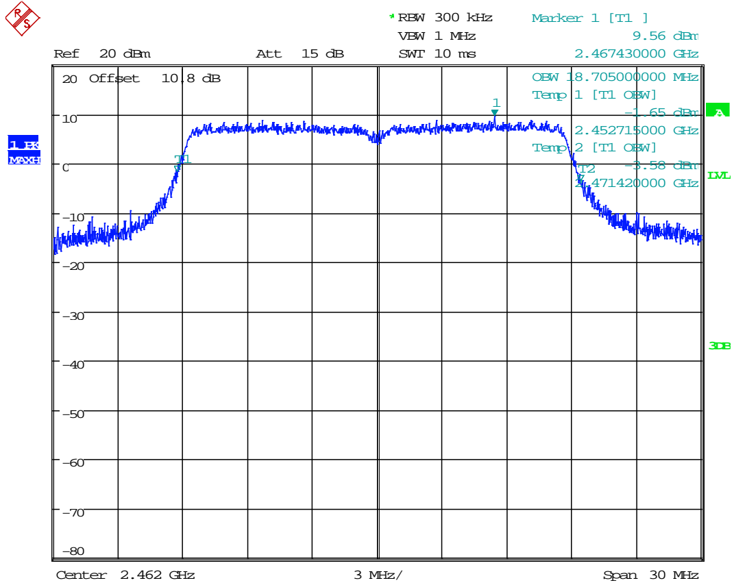
Plot 1.21 – 99% Bandwidth
