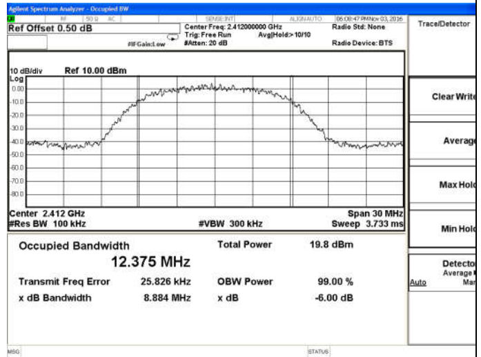
802.11b-Low channel
