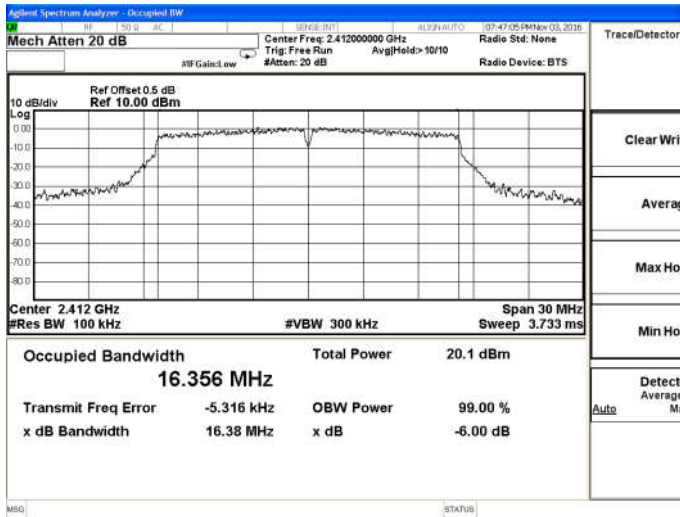
802.11g-Low channel
