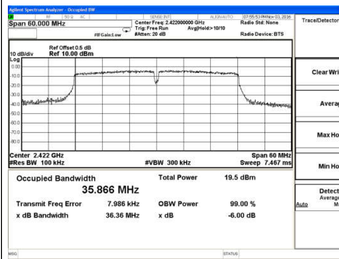
802.11n(HT40)-Low channel
