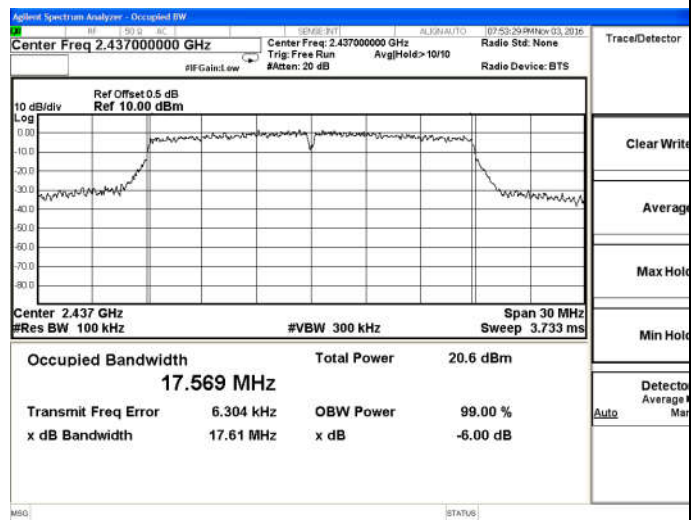
802.11n(HT20)-Middle channel
