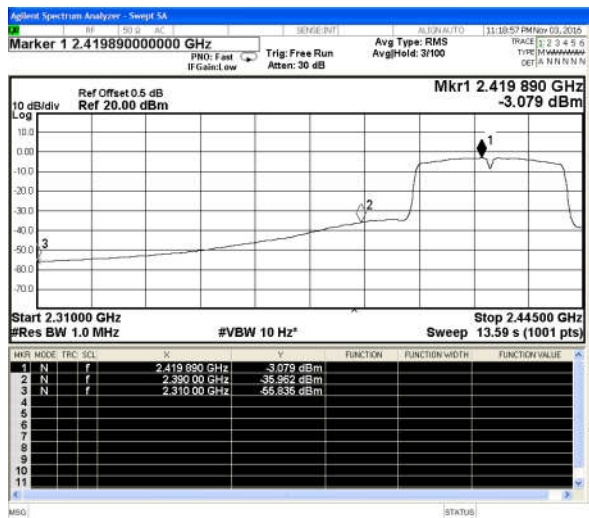
802.11n(HT40)-Low channel(Average)
