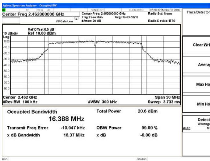
802.11g-High channel
