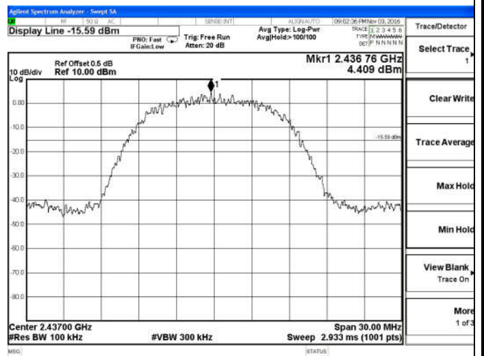
802.11b-Middle channel
