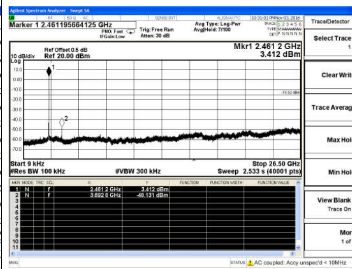
High channel
