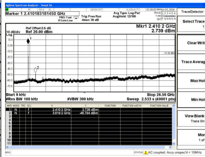
Low channel
