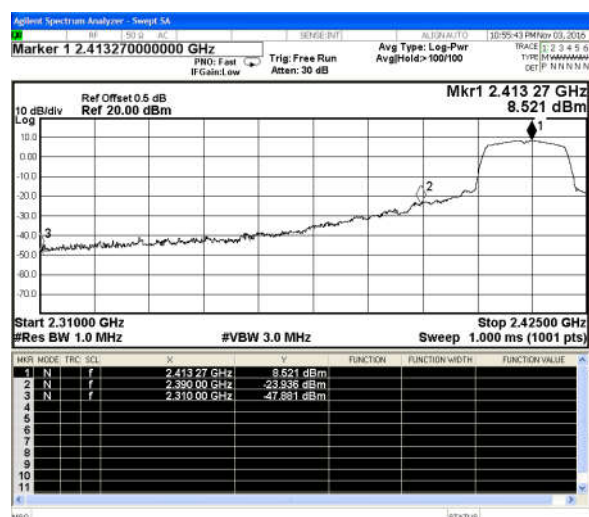
802.11n(HT20)-Low channel(Peak)
