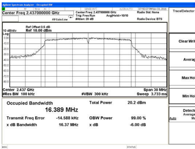
802.11g-Middle channel
