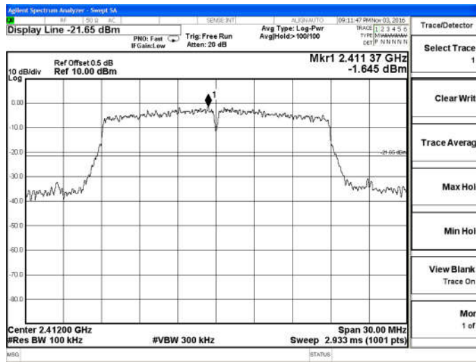
802.11n(HT20)-Low channel
