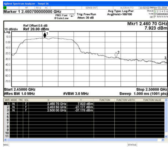
802.11g-High channel(Peak)
