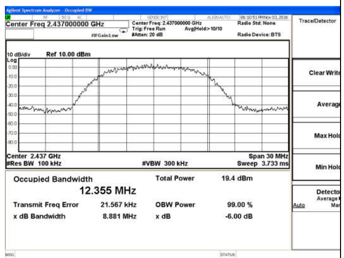
802.11b-Middle channel
