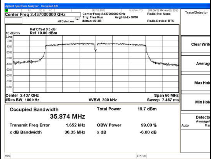
802.11n(HT40)-Mid channel
