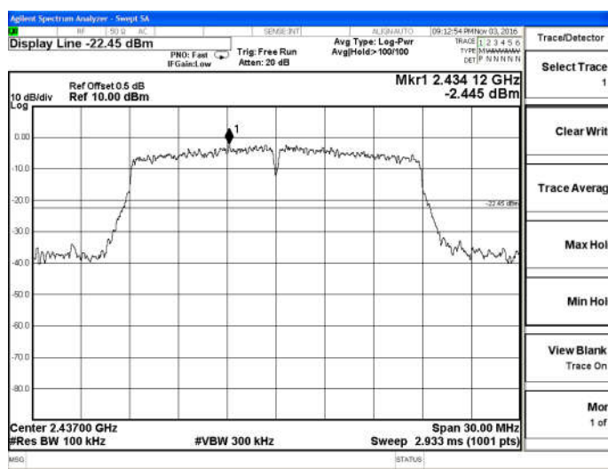
802.11n(HT20)-Middle channel
