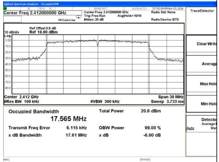
802.11n(HT20)-Low channel
