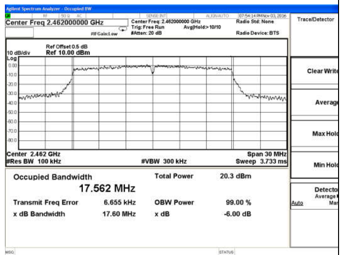
802.11n(HT20)-High channel
