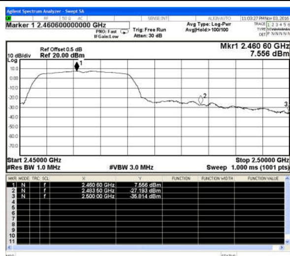
802.11n(HT20)-High channel(Peak)
