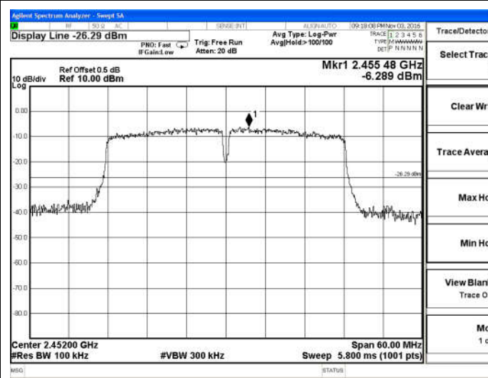
802.11n(HT40)-High channel
