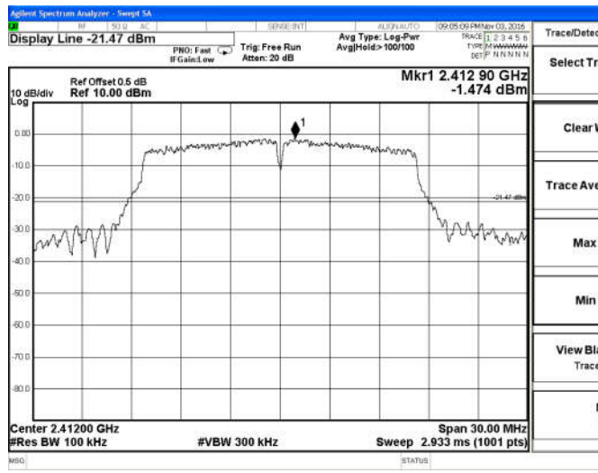
802.11g-Low channel
