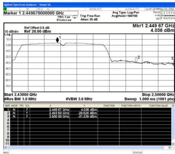
802.11n(HT40)-High channel(Peak)
