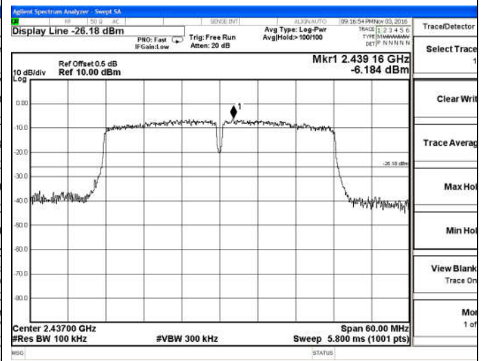
802.11n(HT40)-Mid channel
