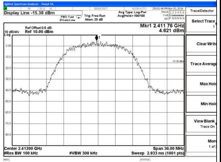
802.11b-Low channel
