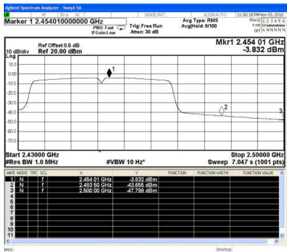
802.11n(HT40)-High channel(Average)
