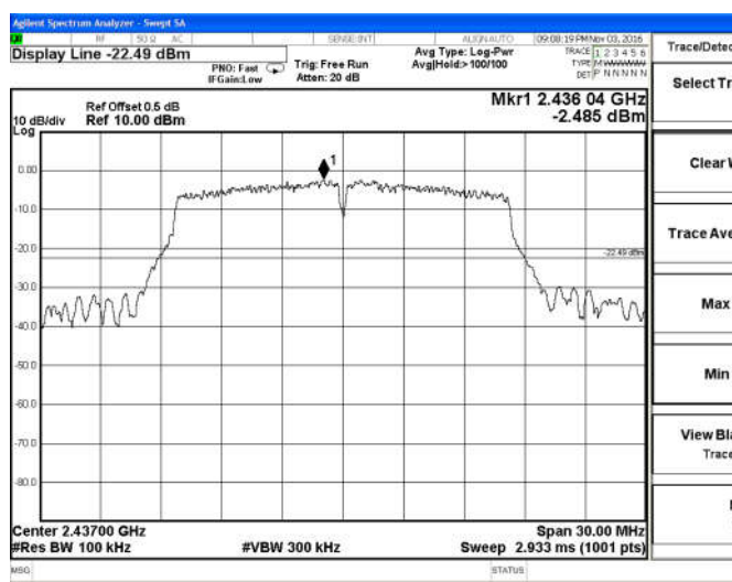
802.11g-Middle channel
