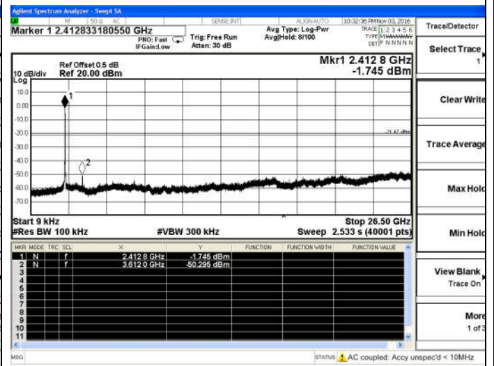
Low channel
