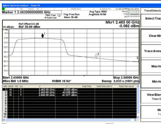
802.11n(HT20)-High channel(Average)
