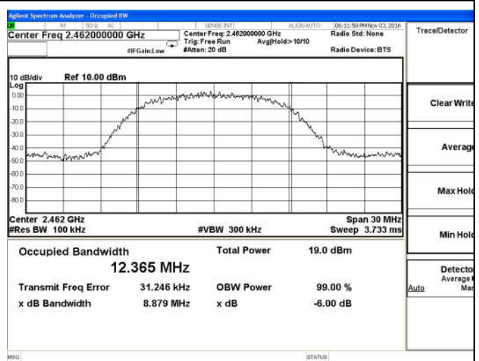
802.11b-High channel
