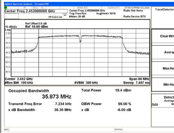
802.11n(HT40)-High channel
