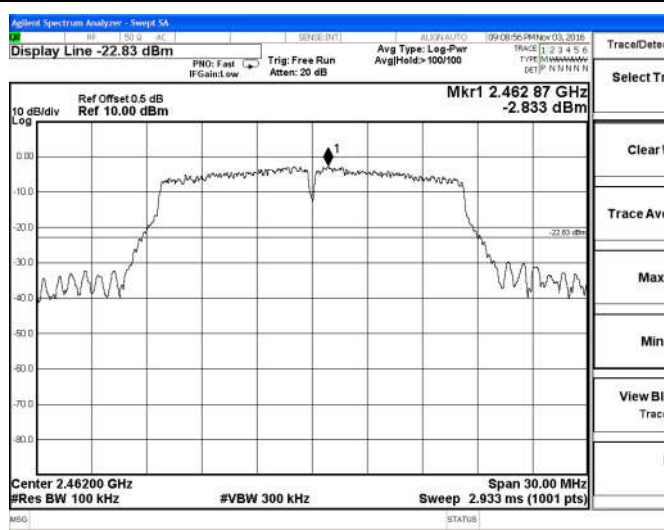
802.11g-High channel
