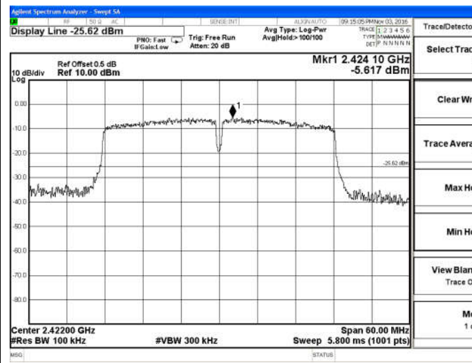
802.11n(HT40)-Low channel
