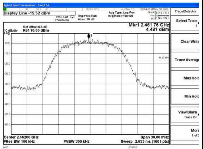
802.11b-High channel
