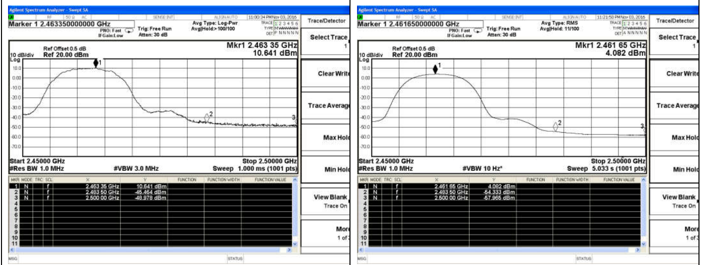
802.11b-High channel(Peak)
