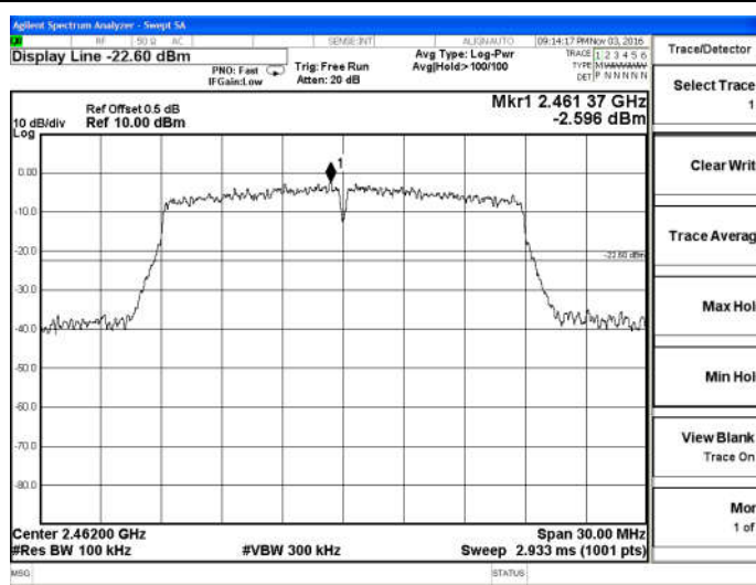
802.11n(HT20)-High channel
