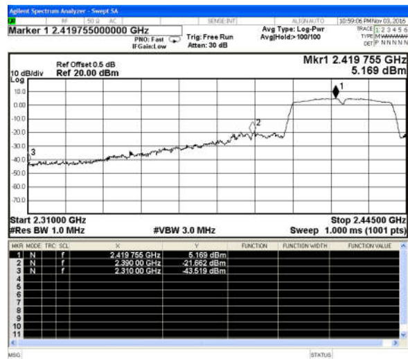
802.11n(HT40)-Low channel(Peak)
