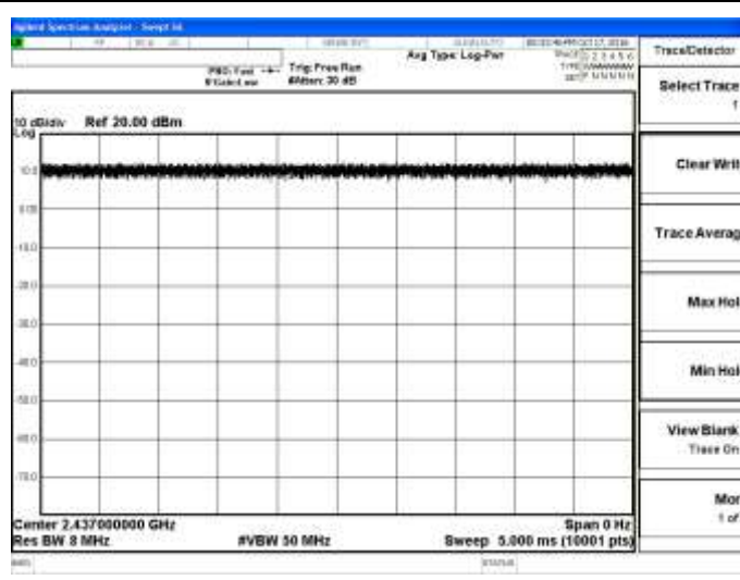
802.11g
