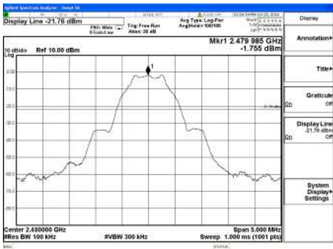
BLE 4.0-High channel Reference
