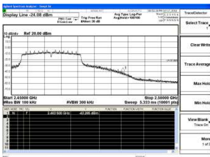
802.11n(HT20)-High channel
