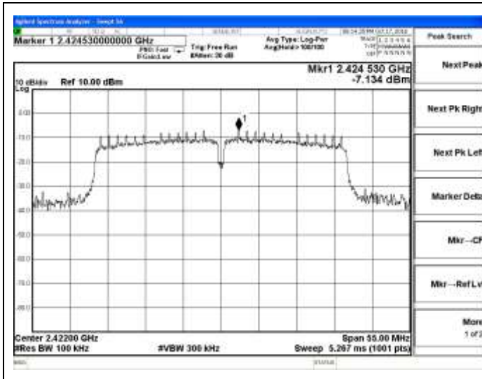
802.11n-HT40 Low channel
