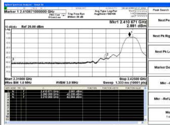
802.11b Low channel(Peak)
