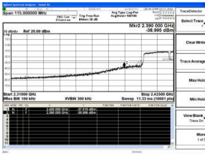
802.11n(HT40)-Low channel
