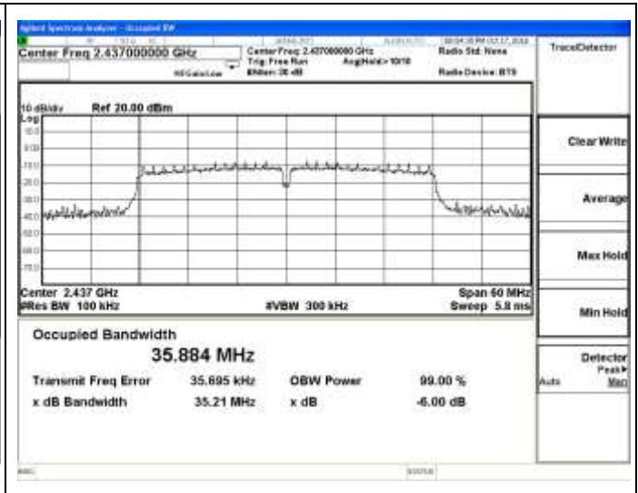
802.11n-HT40 Middle channel
