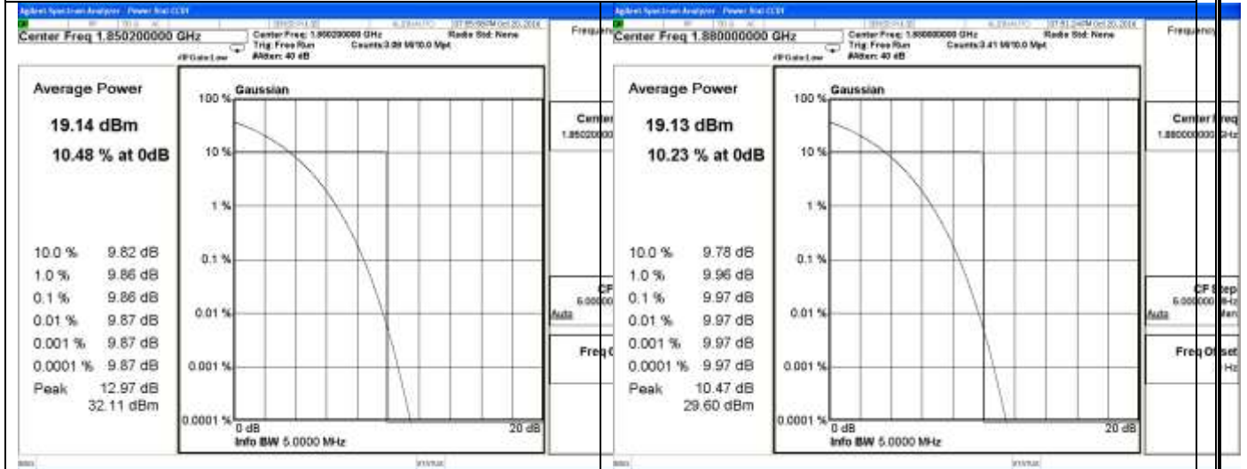
Channel 512 / 1850.2 MHz
