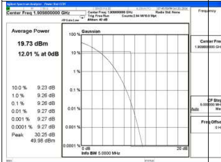
Channel 810 / 1909.8 MHz
