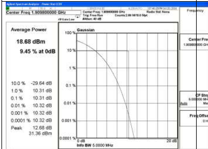
Channel 810 / 1909.8 MHz
