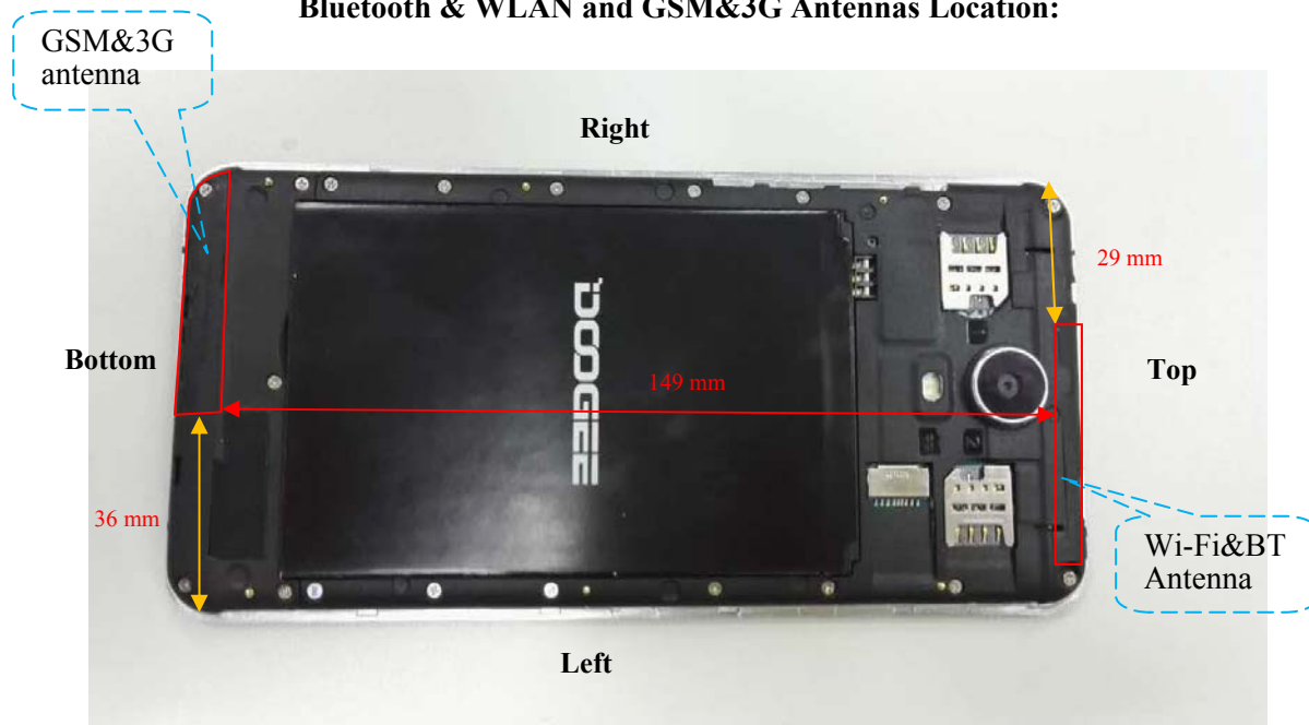
Bluetooth & WLAN and GSM&3G Antennas Location:
