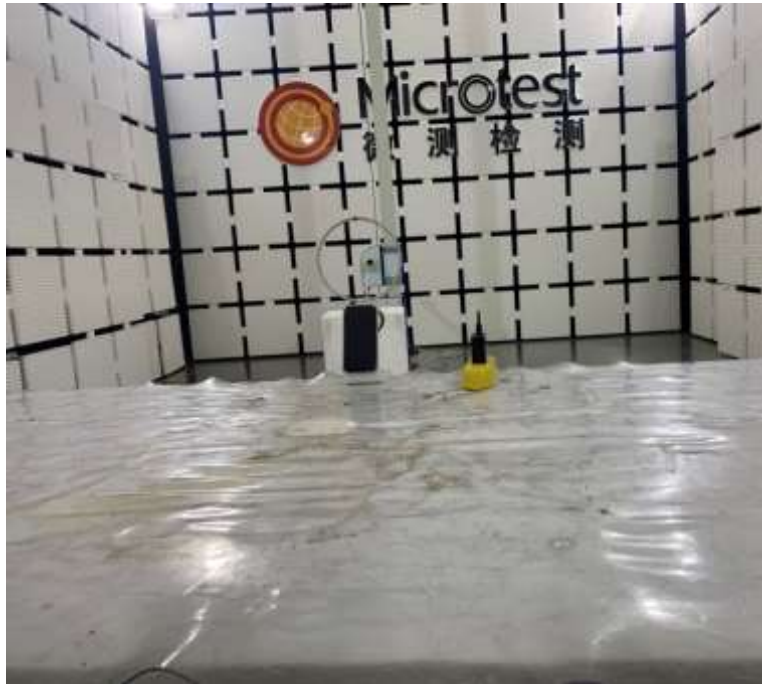
Radiated emissions – Below 30 MHz
