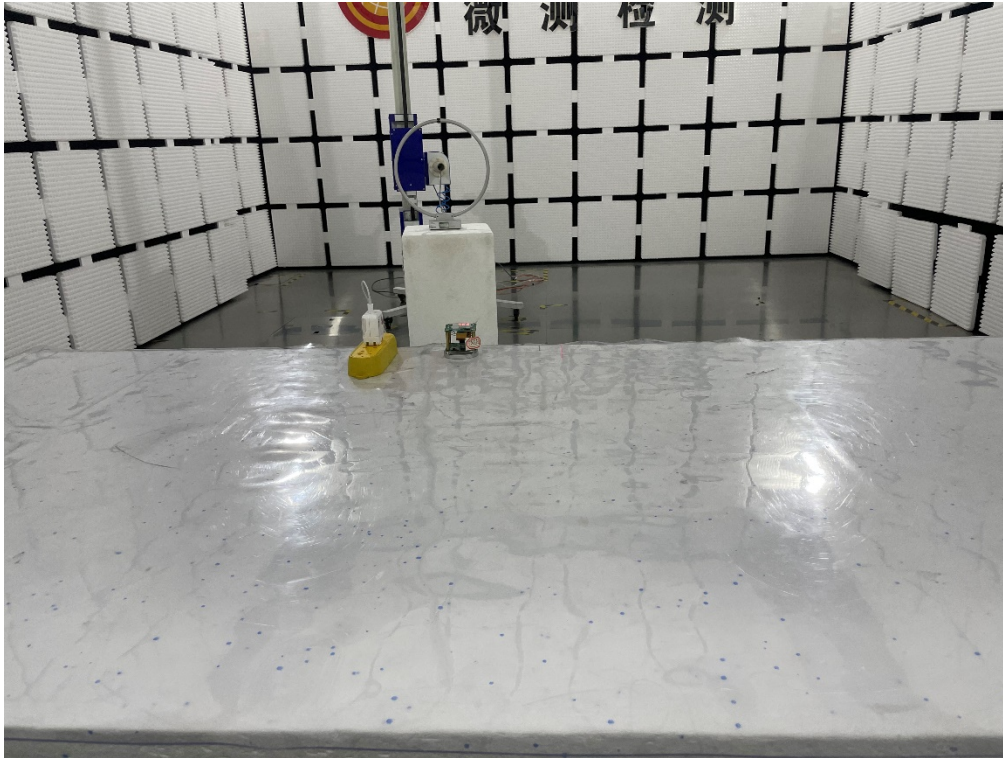
Radiated emissions – Blew 30 MHz
