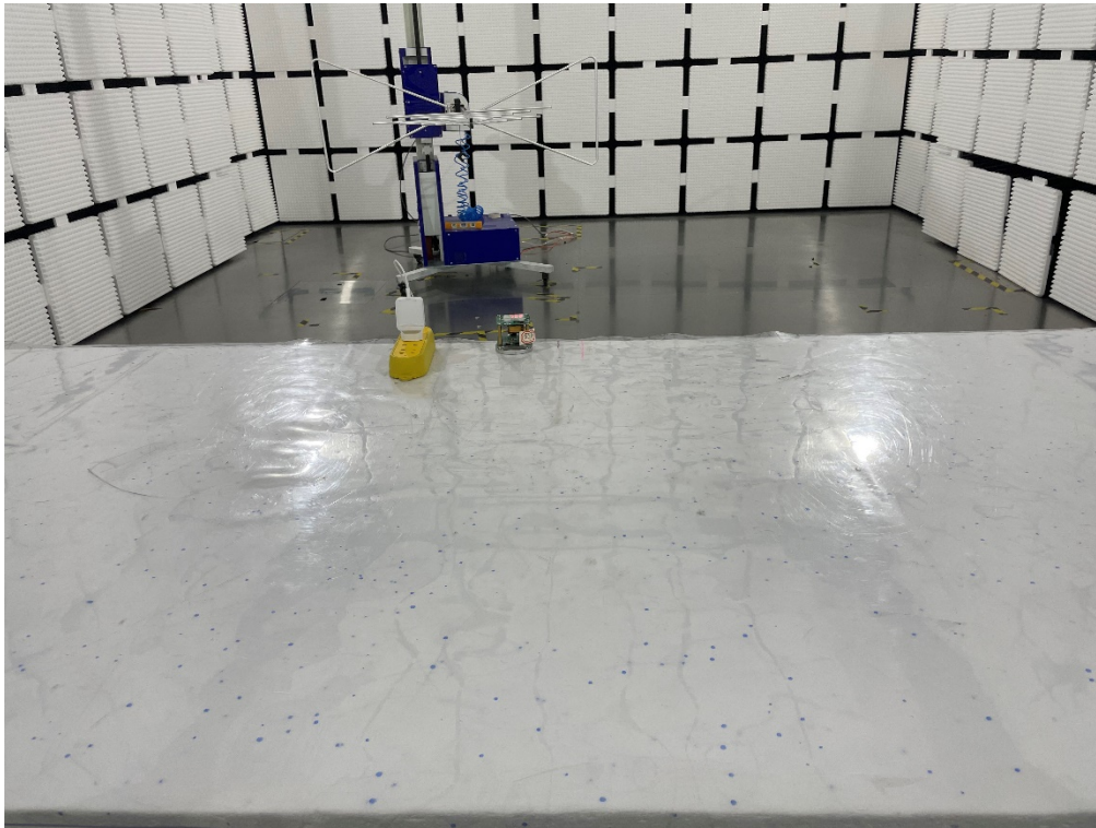
Radiated emissions – Blew 1 GHz
