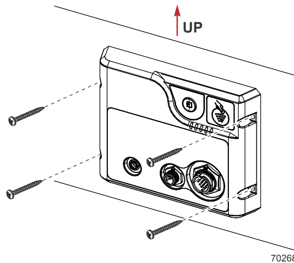
Recommended mounting orientation
