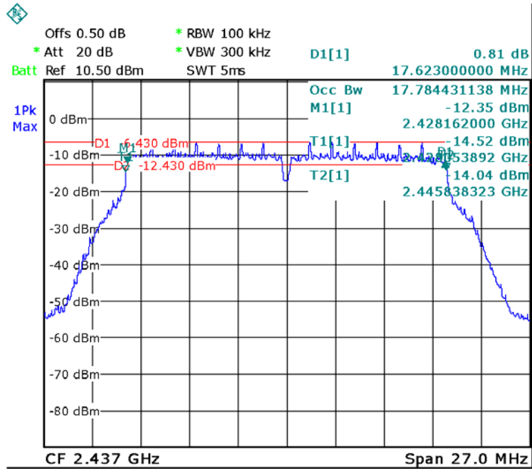
ANT1 TX 11n HT20 Middle channel
