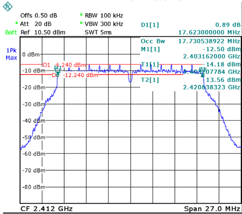
ANT1 TX 11n HT20 Low channel
