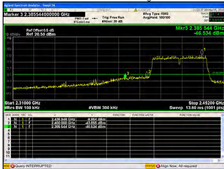
ANT0 TX 11n HT40: Band edge-left side
