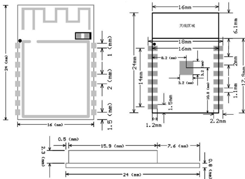
Figure 4 Module Dimensions
