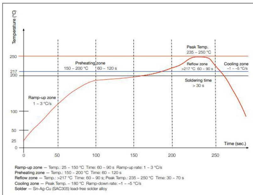
Figure 5 Reflow Profile
