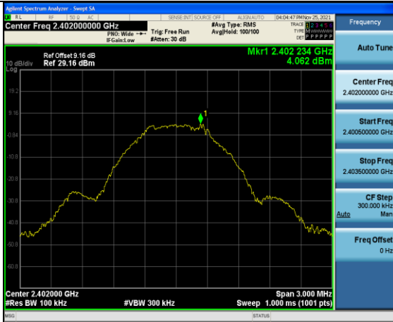
GFSK on Channel 00
