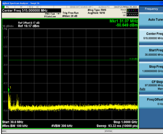
GFSK on Channel 19
