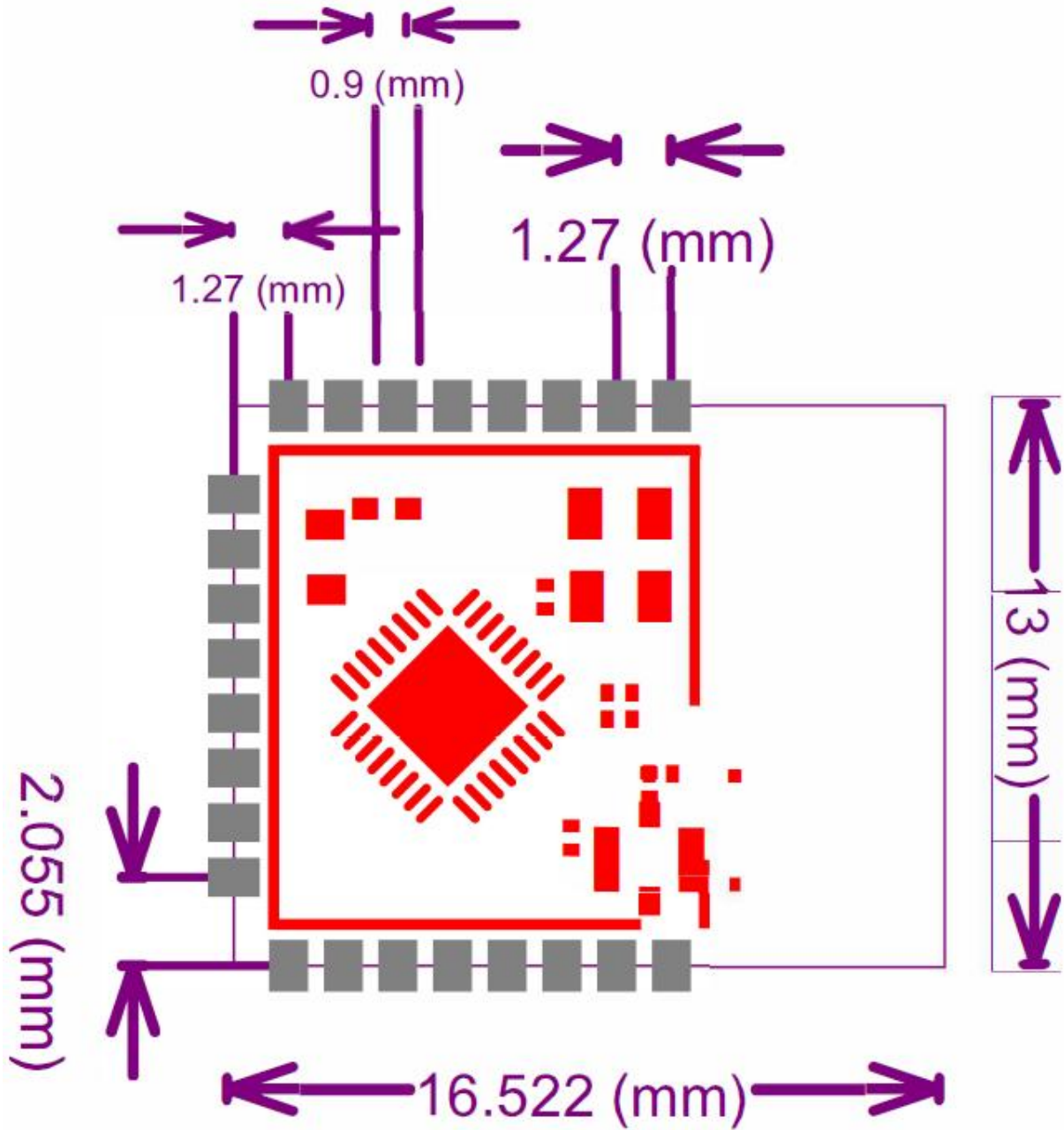
Figure 1 Module Dimensions
