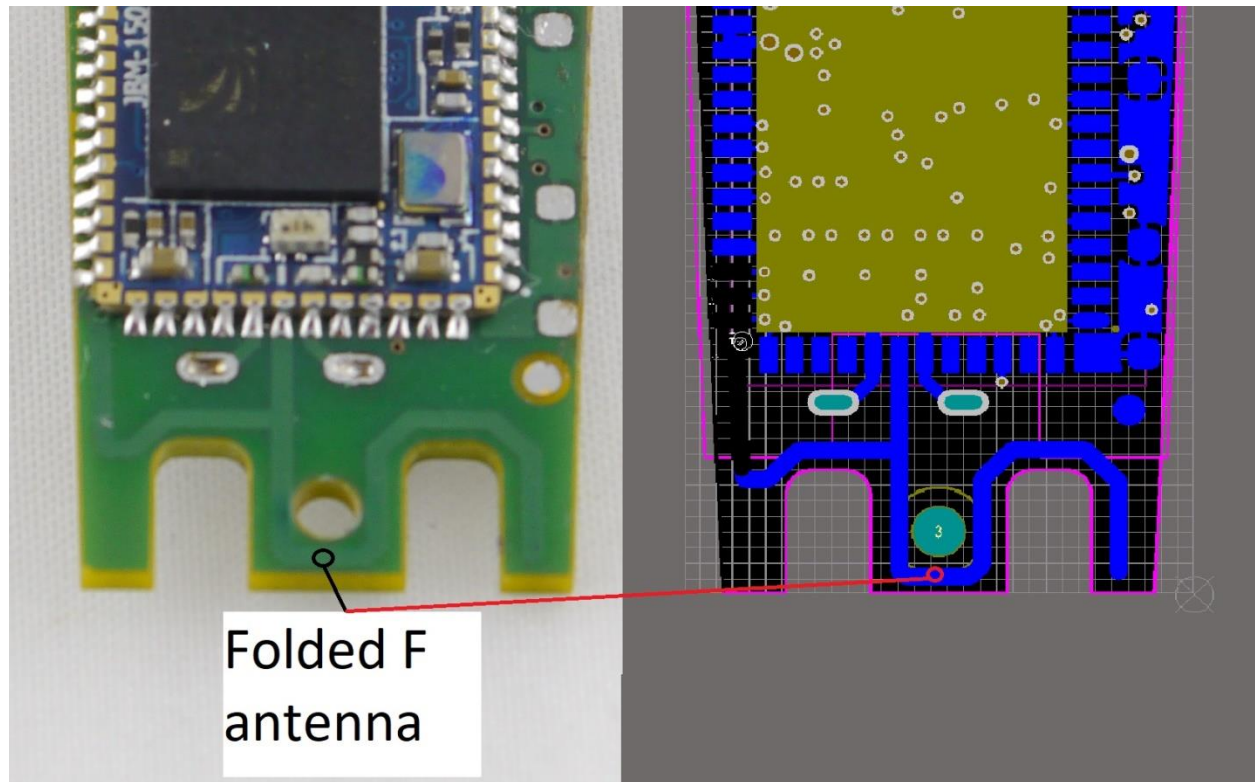
Figure 1: Closeup of printed antenna
