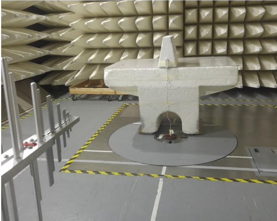
Photograph No.2 Setup for carrier field strength measurements in the anechoic chamber in 30 – 1000 MHz range
