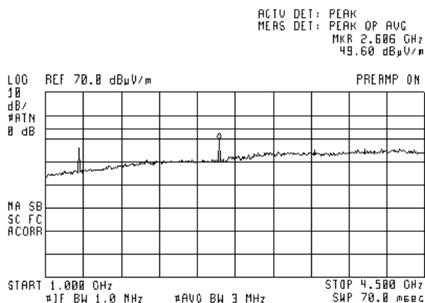
Plot 7.2.12 Radiated emission measurements from 1000 to 4500 MHz
