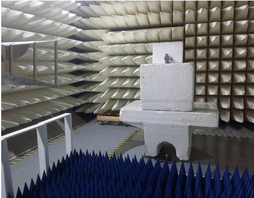
Photograph No.3 Setup for spurious emission field strength measurements in the anechoic chamber above 1000 MHz range
