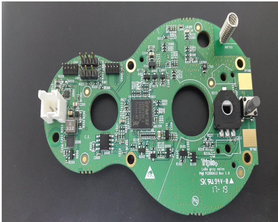
Photograph No.2 Actuator shut off unit PCB front view
