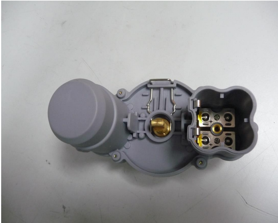
Photograph No.3 Actuator shut off unit bottom view
