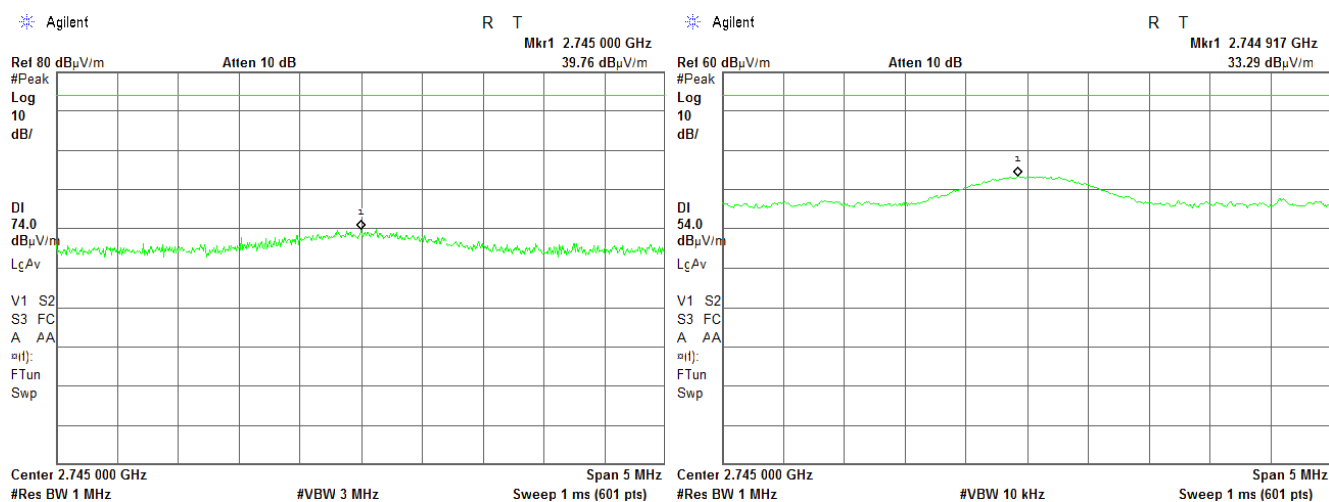
Plot 7.2.14 Radiated emission measurements at the third harmonic frequency
