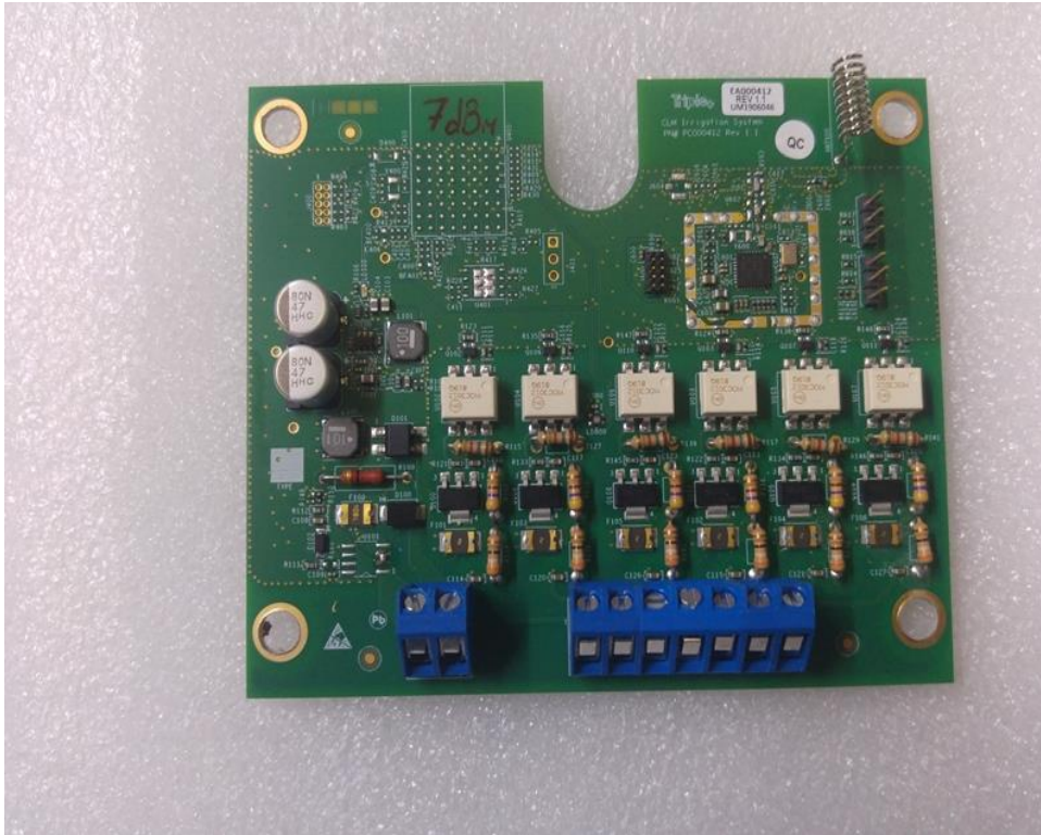
Photograph No.2 Irrigation Controller unit PCB front view
