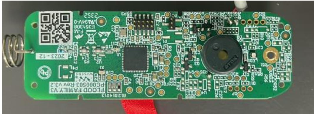
Photograph No.7 Flood family (Universal Switch) Model Name CBM-RMAMAP-5 unit internal view
