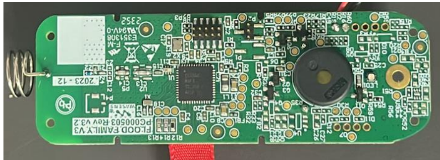
Photograph No.3 Flood family (Universal Switch) Model Name CBM-FDAMAP-5 unit internal view
