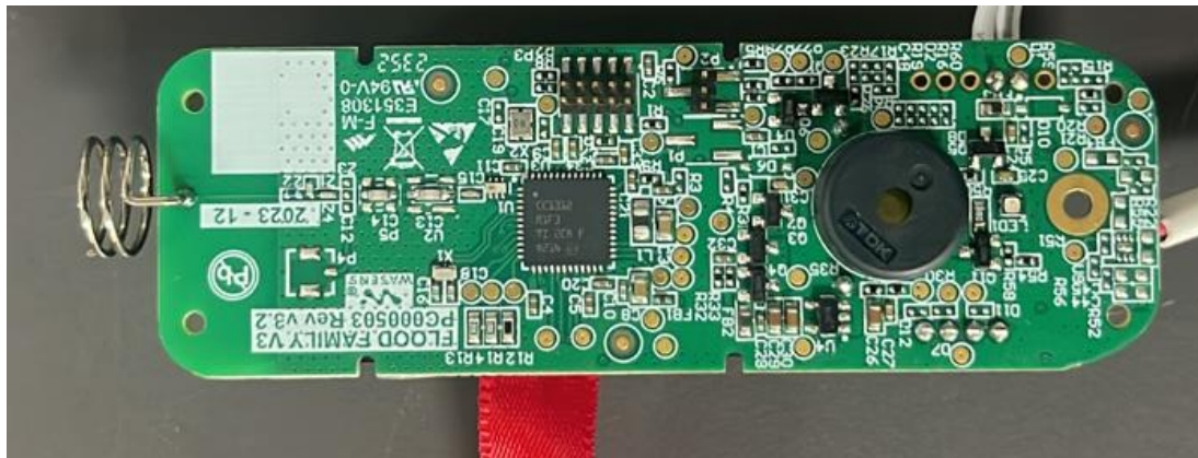
Photograph No.13 Flood family (Universal Switch) Model Name CBM-BHAMAP-5 unit internal view
