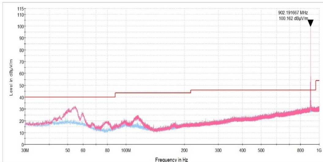
Plot 7.6.5 Radiated emission measurements from 30 to 1000 MHz at the mid carrier frequency
