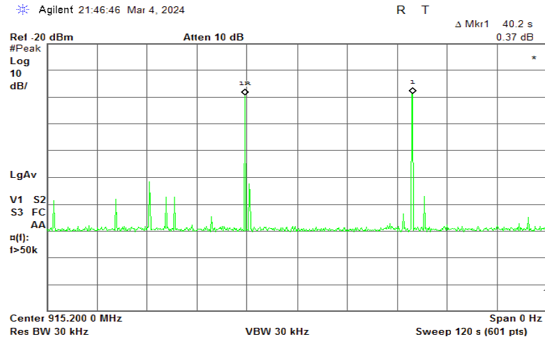
Plot 7.4.2 Transmission pulse period
