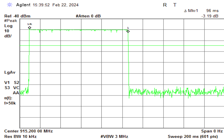
Plot 7.4.1 Single transmission duration
