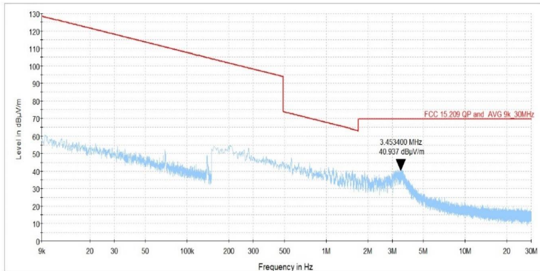
Plot 7.5.2 Radiated emission measurements from 9 to 30 MHz at the mid carrier frequency
