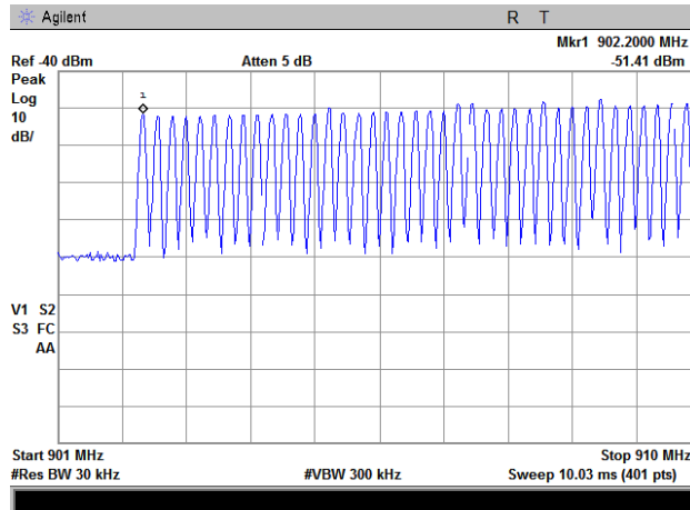
Plot 7.2.1 Number of hopping frequencies
