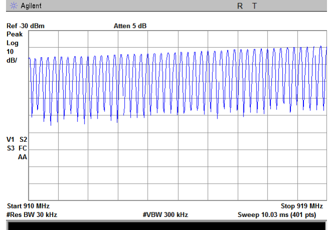
Plot 7.2.1 Number of hopping frequencies
