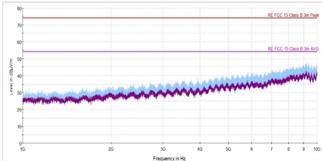
Plot 7.5.8 Radiated emission measurements from 1000 to 10000 MHz at the mid carrier frequency
