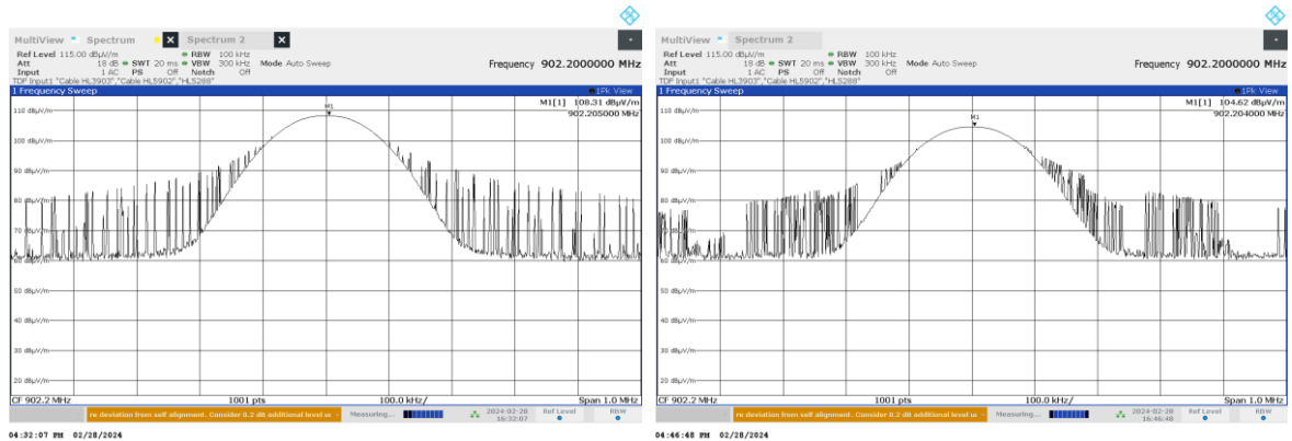
Plot 7.4.1 Field strength of carrier at low frequency
