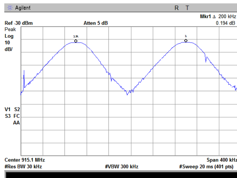
Plot 7.1.1 Carrier frequency separation
