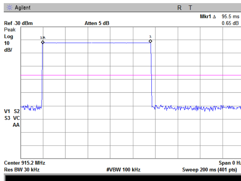
Plot 7.3.1 Single transmission duration
