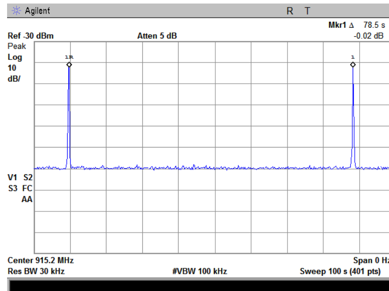
Plot 7.3.2 Transmission pulse period
