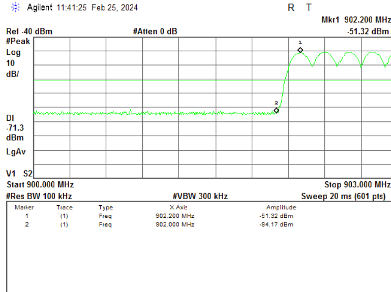
Plot 7.8.5 The highest band edge emission at low carrier frequency with hopping function enabled
