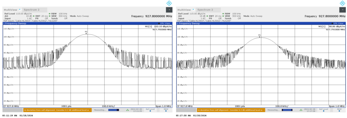
Plot 7.4.3 Field strength of carrier at high frequency
