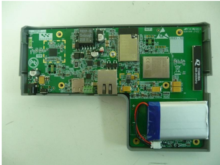
Photograph No.1 Controller unit internal view
