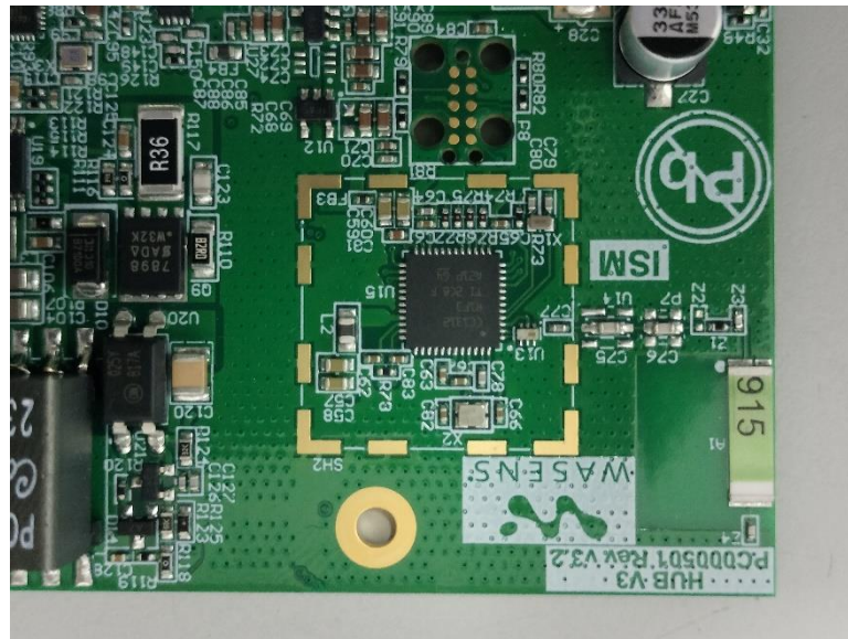
Photograph No.4 Controller unit Print side of the RF PCB
