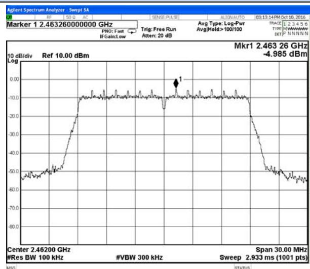
802.11n-HT20 Chain 1-High channel Reference
