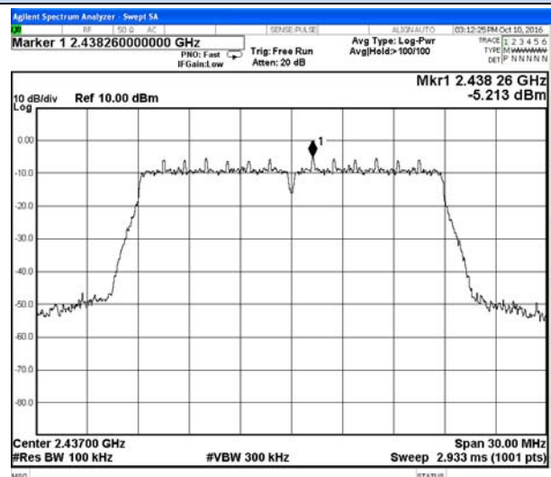
802.11n-HT20 Chain 1-Middle channel Reference
