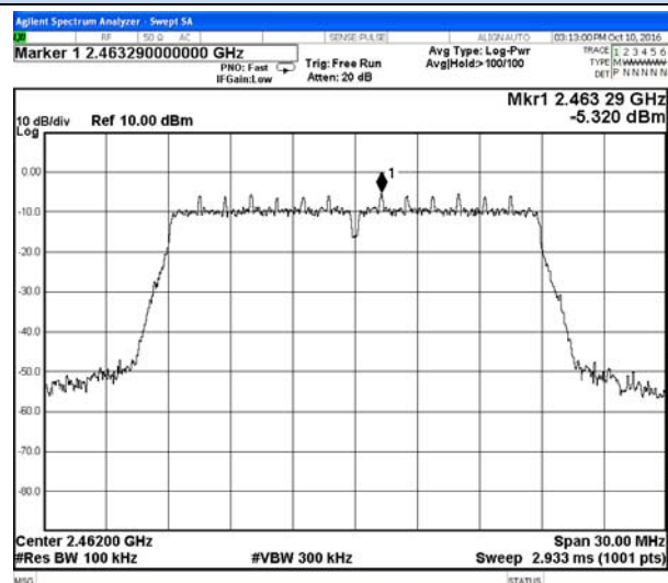
802.11n-HT20 Chain 0-High channel Reference
