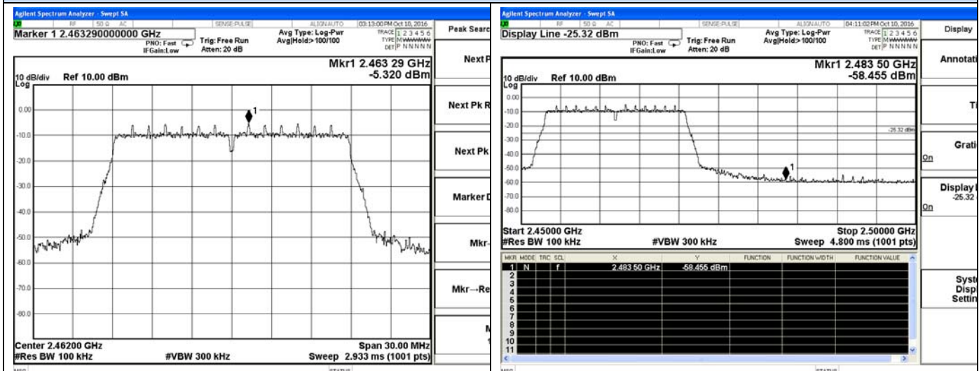
802.11n-HT20 Chain 0-High channel Reference
