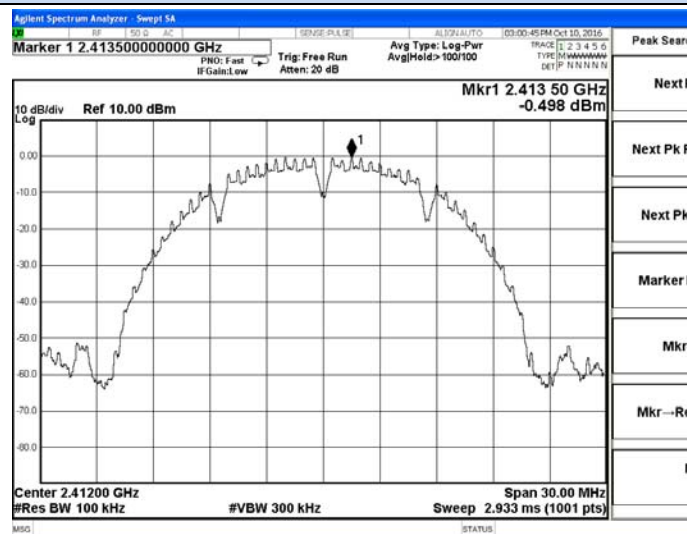
802.11b Chain 1-Low channel
