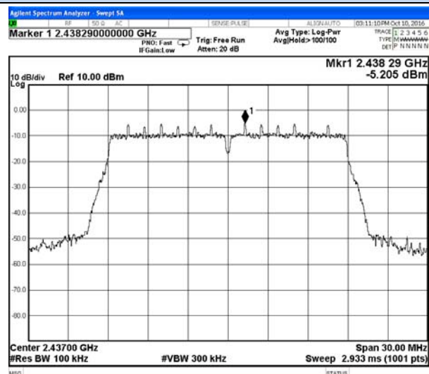
802.11n-HT20 Chain 0-Middle channel Reference
