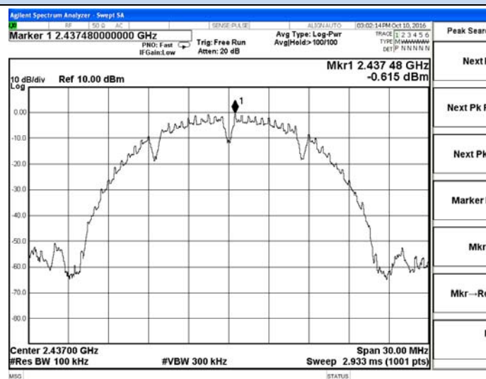
802.11b Chain 1-Middle channel
