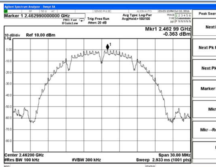
802.11b Chain 1-High channel
