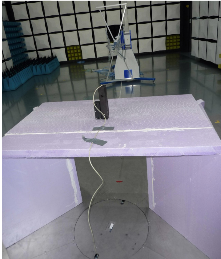
191513SK_03:Final Mesurement 30 – 1000 MHz
