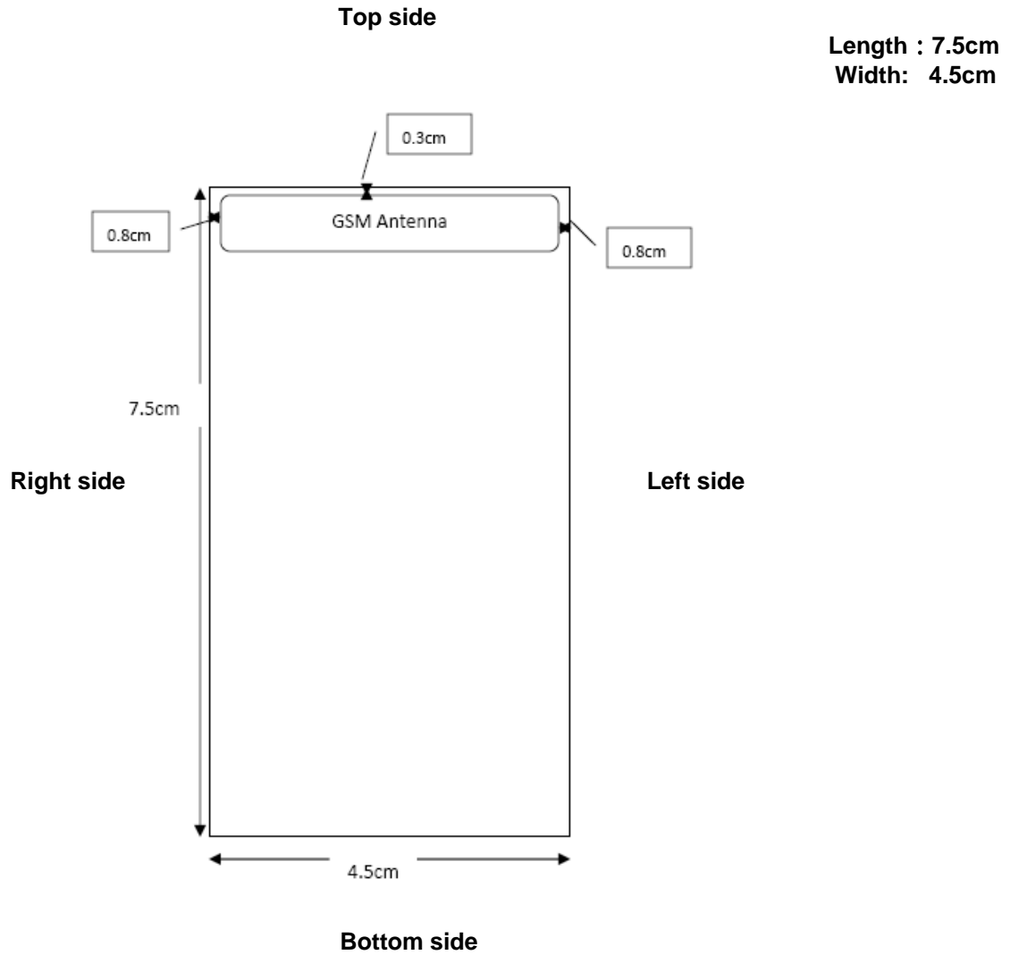
Figure1: The antenna position of the DUT
