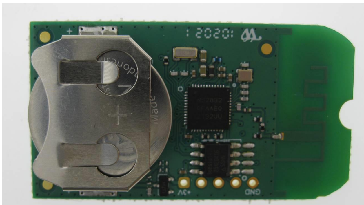
BT HOS DID – PCB front
