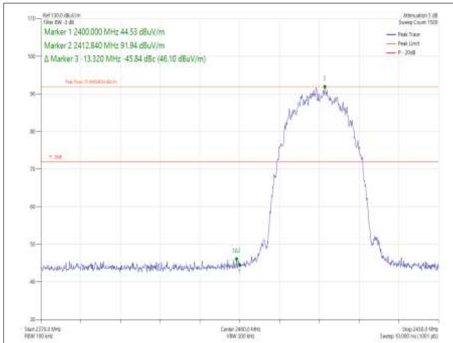
Figure 1 - Data Rate/MCS with the Highest Power - 1 Mbps - 2412 MHz - Band Edge Frequency 2400 MHz
