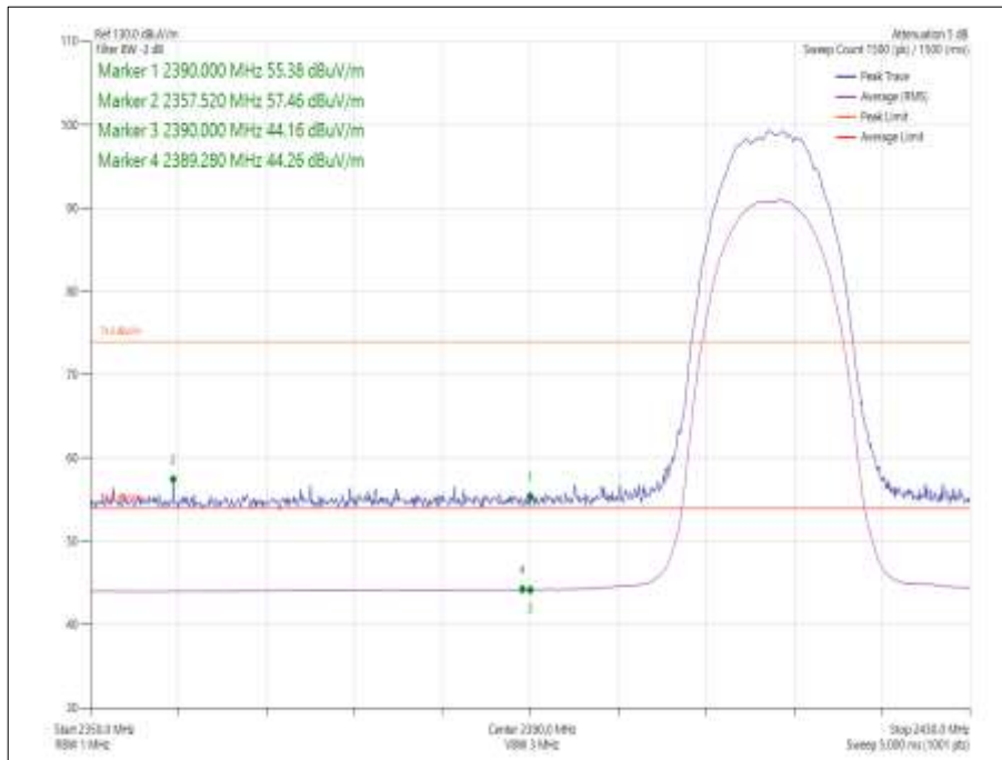
Figure 7 - Data Rate/MCS with the Highest Power - 1 Mbps - 2412 MHz - Band Edge Frequency 2390 MHz
