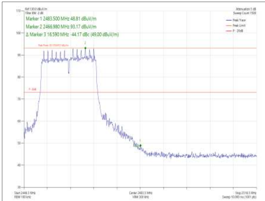
Figure 4 - Data Rate/MCS with the Highest Power - 6 Mbps - 2462 MHz - Band Edge Frequency 2483.5 MHz
