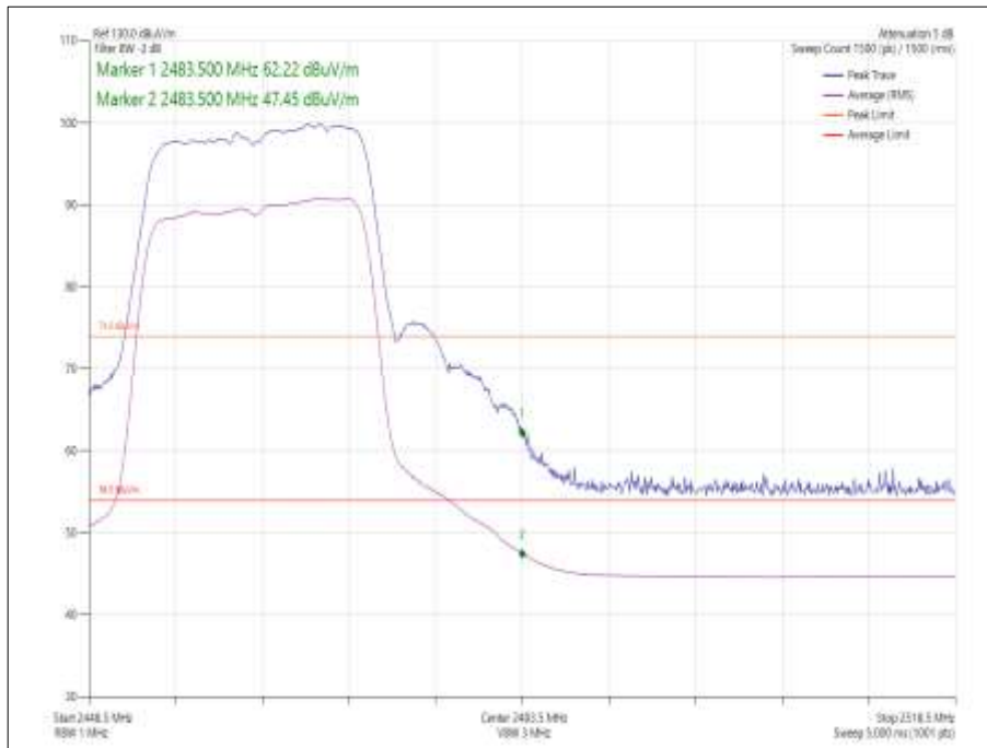
Figure 12 - Data Rate/MCS with the Highest Power - MCS0 - 2462 MHz - Band Edge Frequency 2483.5 MHz
