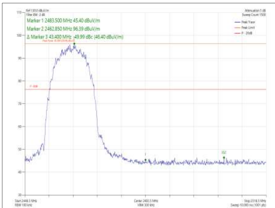
Figure 2 - Data Rate/MCS with the Highest Power - 1 Mbps - 2462 MHz - Band Edge Frequency 2483.5 MHz
