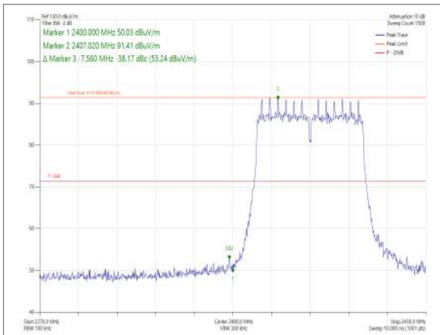
Figure 3 - Data Rate/MCS with the Highest Power - 6 Mbps - 2412 MHz - Band Edge Frequency 2400 MHz
