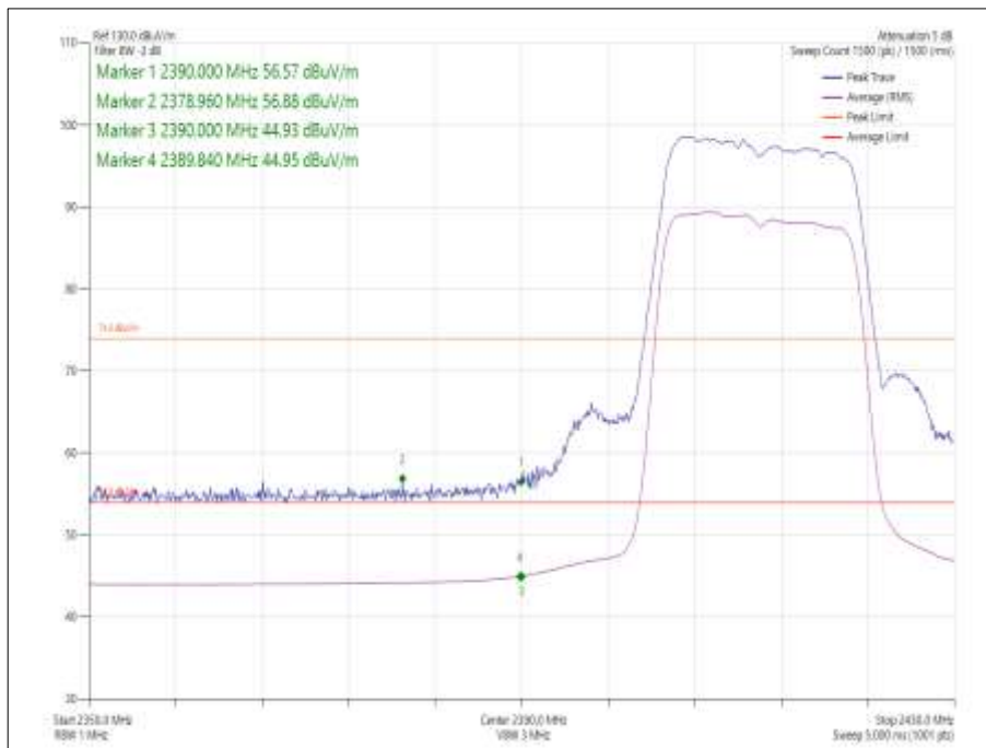
Figure 11 - Data Rate/MCS with the Highest Power - MCS0 - 2412 MHz - Band Edge Frequency 2390 MHz
