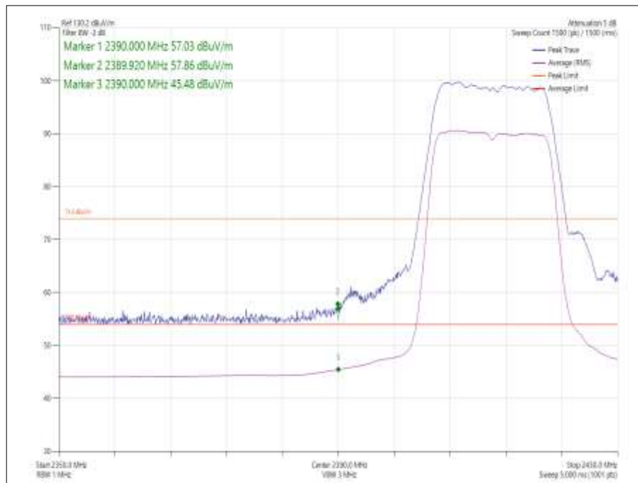
Figure 9 - Data Rate/MCS with the Highest Power - 6 Mbps - 2412 MHz - Band Edge Frequency 2390 MHz
