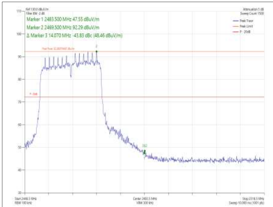
Figure 6 - Data Rate/MCS with the Highest Power - MCS0 - 2462 MHz - Band Edge Frequency 2483.5 MHz
