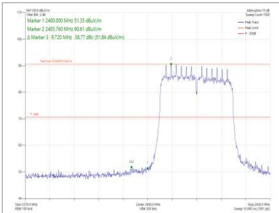
Figure 5 - Data Rate/MCS with the Highest Power - MCS0 - 2412 MHz - Band Edge Frequency 2400 MHz
