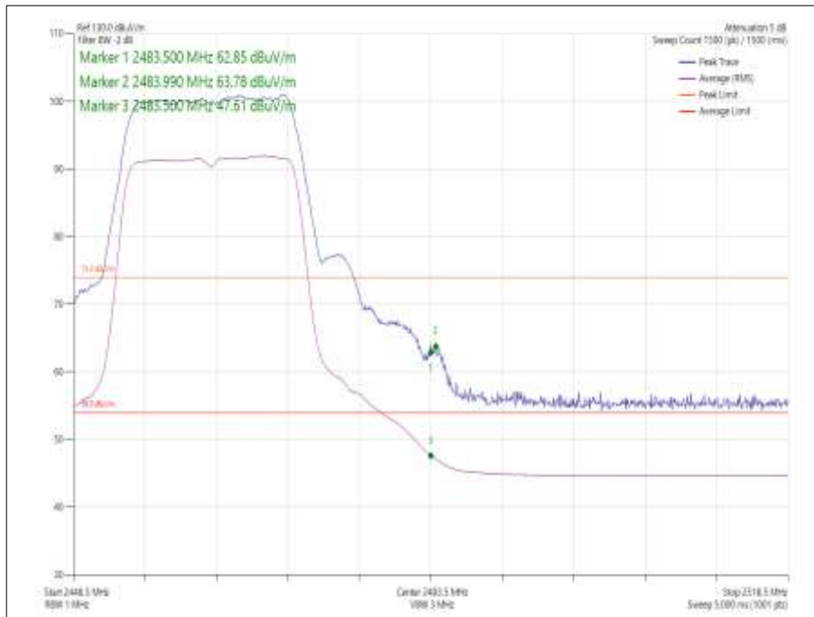
Figure 10 - Data Rate/MCS with the Highest Power - 6 Mbps - 2462 MHz - Band Edge Frequency 2483.5 MHz
