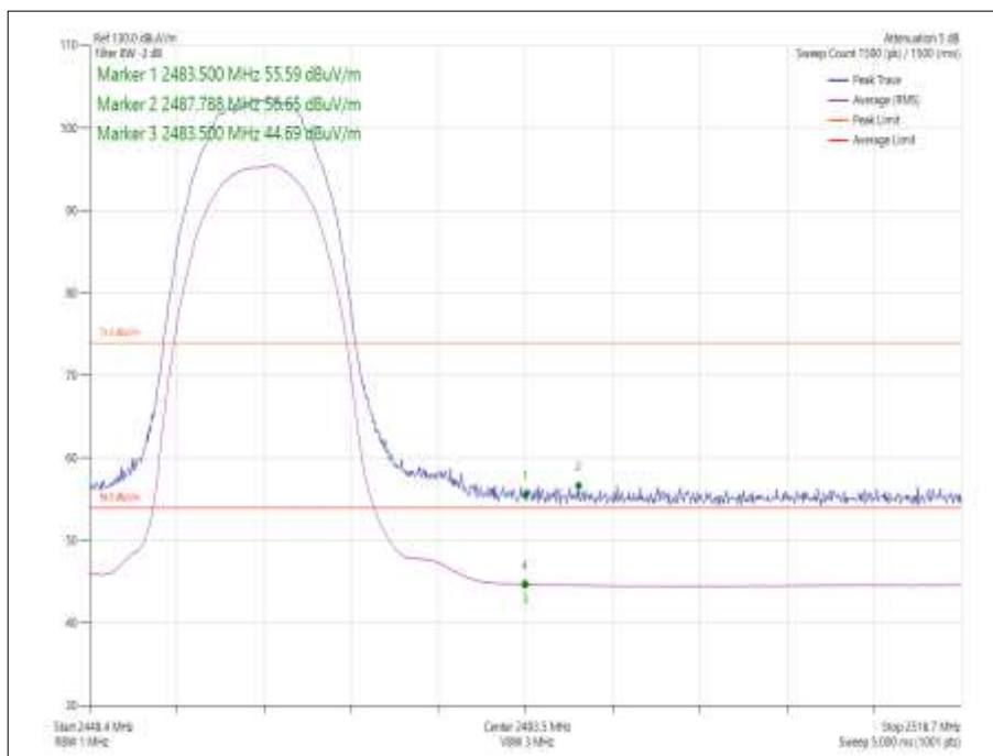
Figure 8 - Data Rate/MCS with the Highest Power - 1 Mbps - 2462 MHz - Band Edge Frequency 2483.5 MHz
