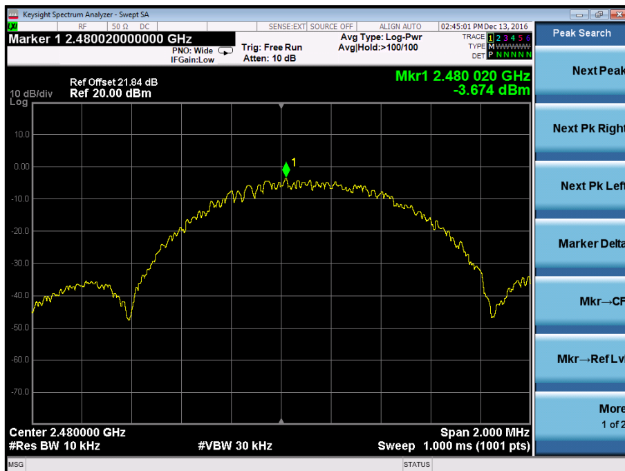
Figure 27 - 2480 MHz
