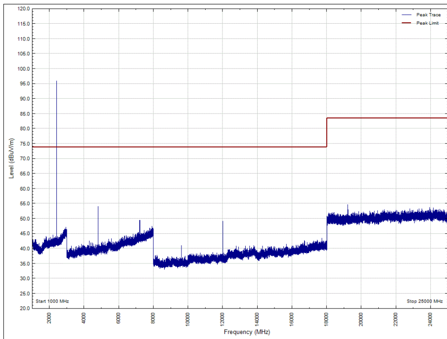
Figure 17 - 2402 MHz, 1 GHz to 25 GHz, Horizontal, Y Orientation: - Peak
