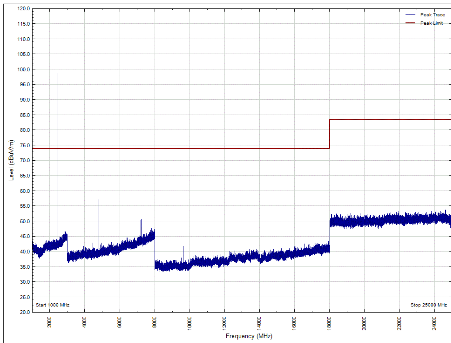
Figure 15 - 2402 MHz, 1 GHz to 25 GHz, Vertical, Y Orientation: - Peak
