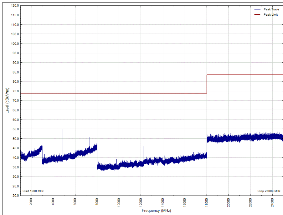
Figure 37 - 2440 MHz - 1 GHz to 25 GHz, Vertical, EUT Orientation: Z, Peak
