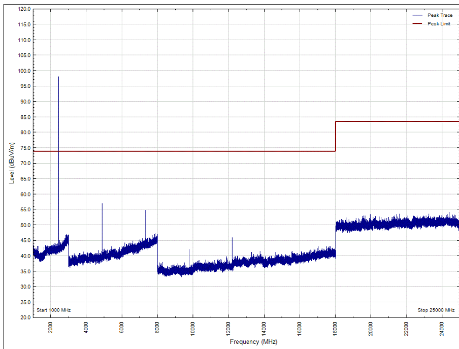
Figure 39 - 2440 MHz - 1 GHz to 25 GHz, Horizontal, EUT Orientation: Z, Peak
