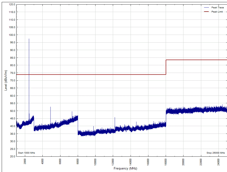
Figure 35 - 2440 MHz - 1 GHz to 25 GHz, Horizontal, EUT Orientation: Y, Peak
