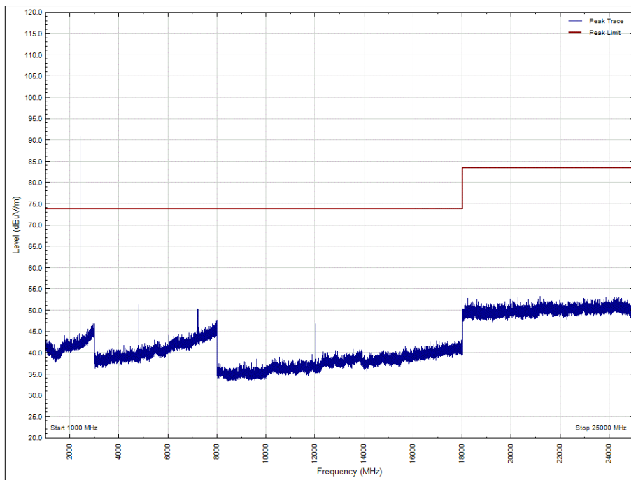
Figure 11 - 2402 MHz, 1 GHz to 25 GHz, Vertical, X Orientation: - Peak
