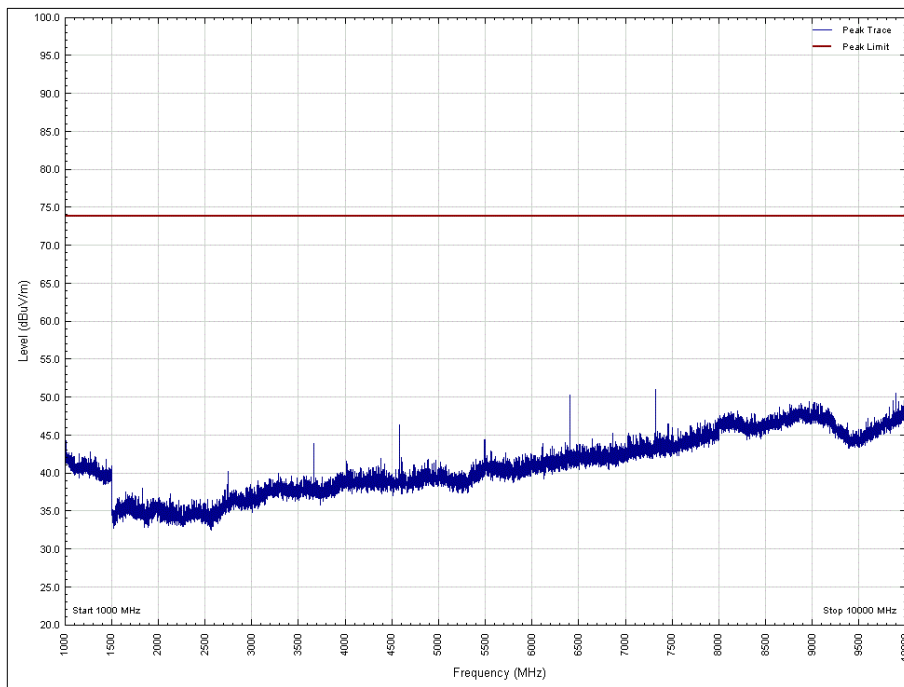
Figure 34 - 915.0 MHz - 1 GHz to 10 GHz, Horizontal, EUT Orientation: X, Peak
